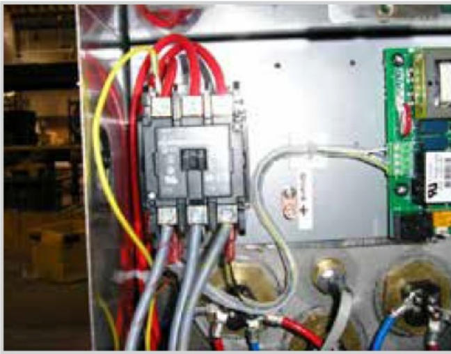
Showing booster contactor, yellow signal wire
