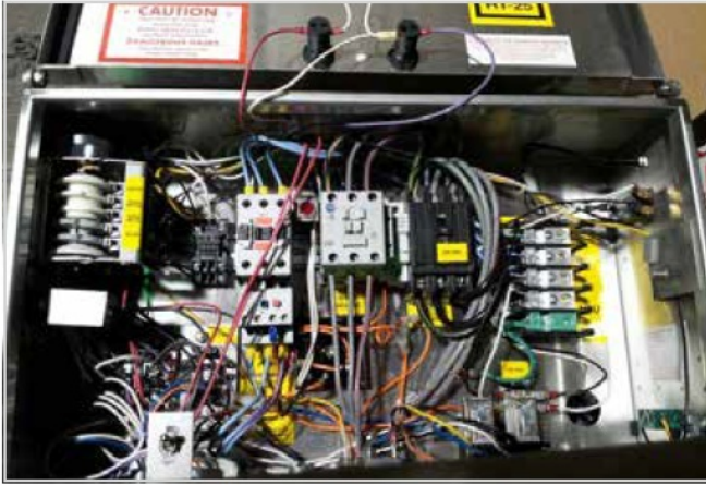
Showing HT-25, 5-wire control box
