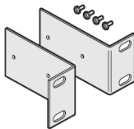
19" rack-mount kit Part number: RMK14
