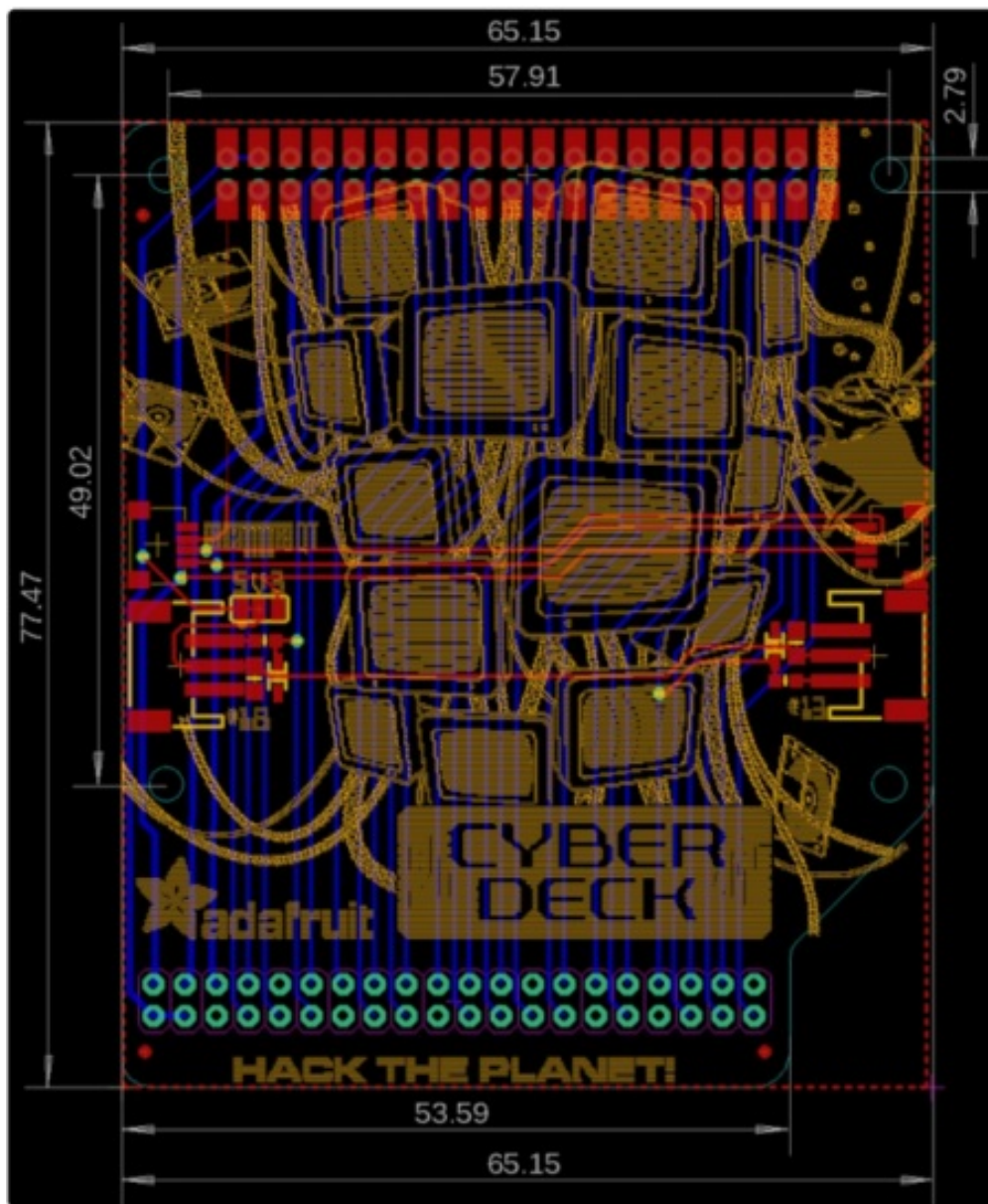
Schematic and Fab Print for CYBERDECK Bonnet
