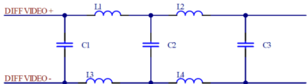
Figure 4: Low Pass Filter Design
