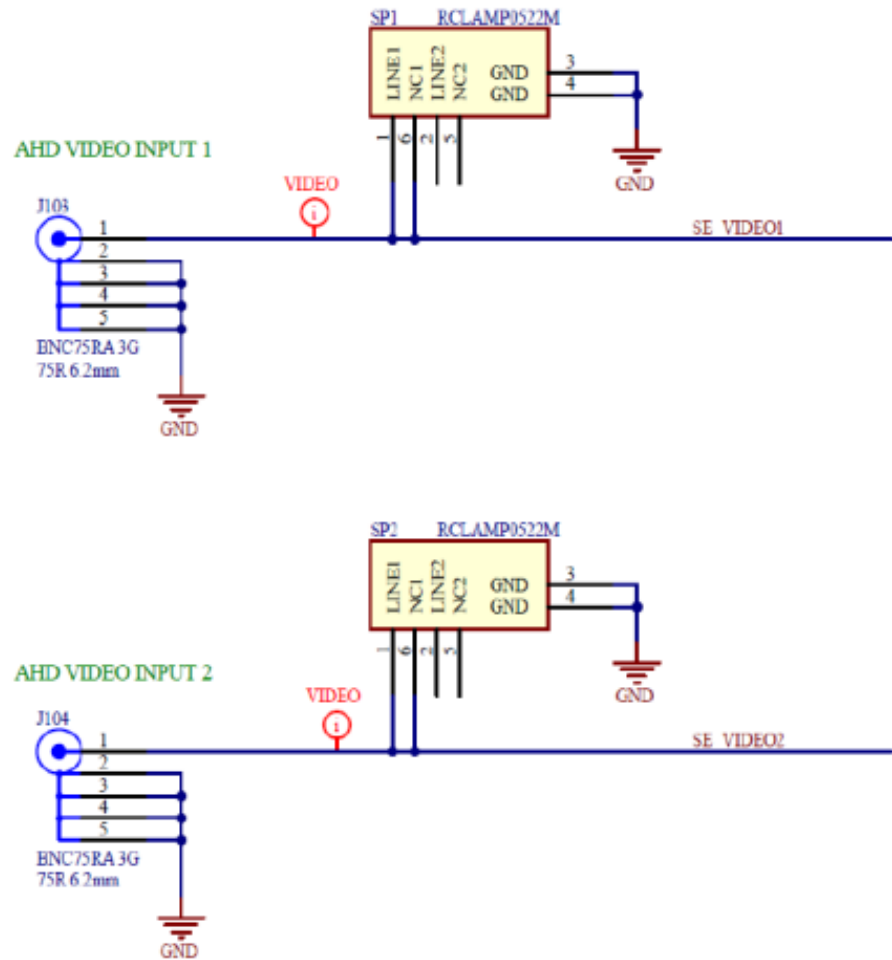
Figure 2: BlueBird Analog - SDI Adaptor Evaluation board single ended input circuits
