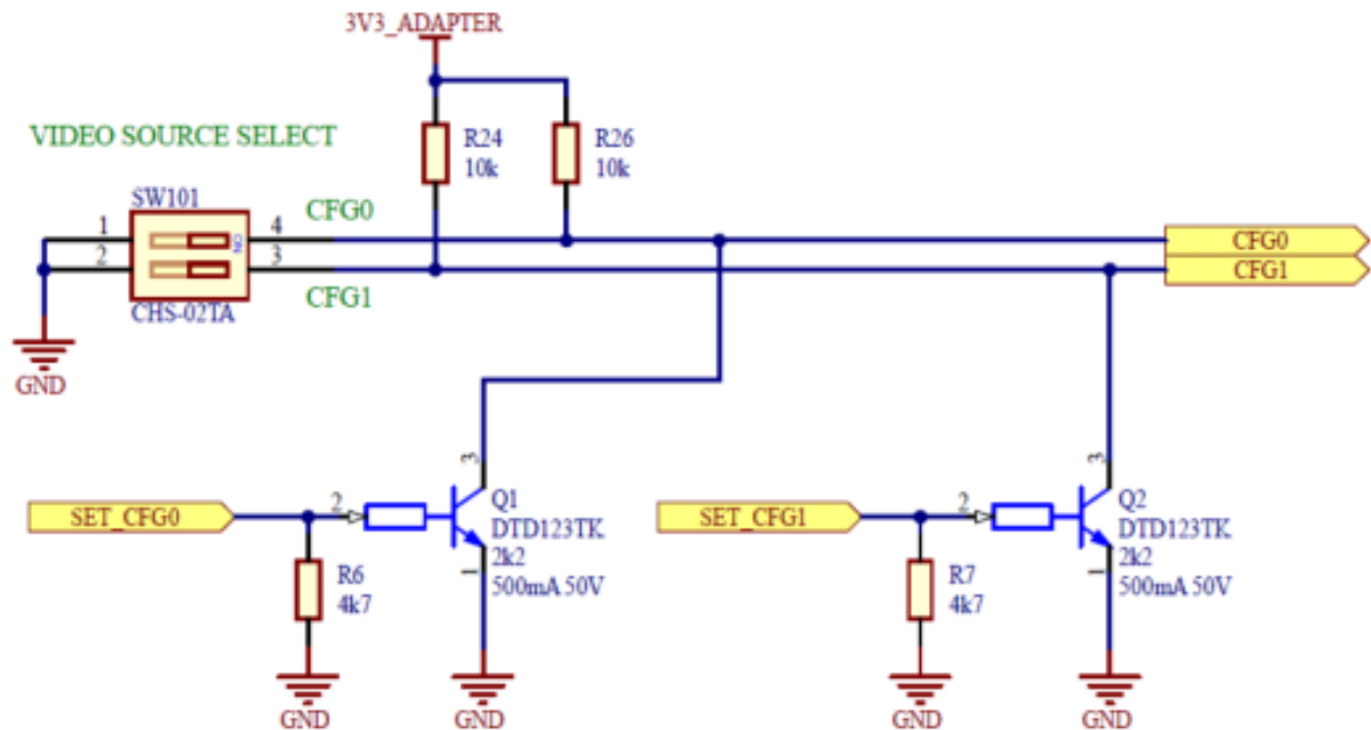
Figure 6: BlueBird Analog - SDI Evaluation Board configuration signal circuit
