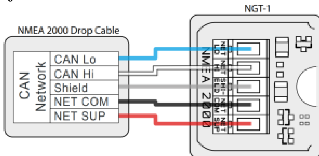
Figure 4 – NMEA 2000 PCB Connections
