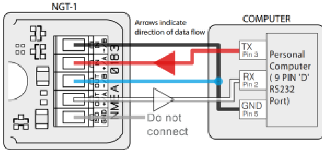
Figure 3 – PC / RS232 Port Connections
