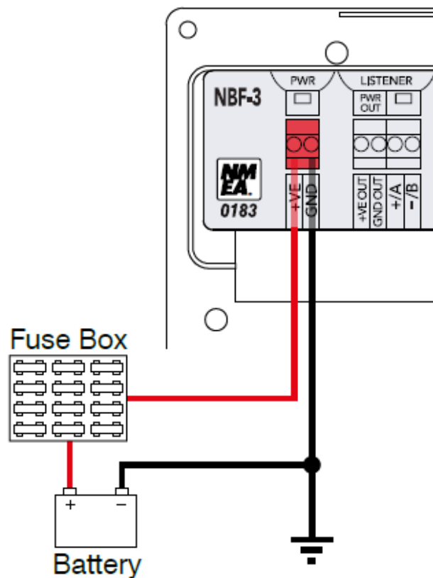
Figure 3 - Power Connection Diagram
