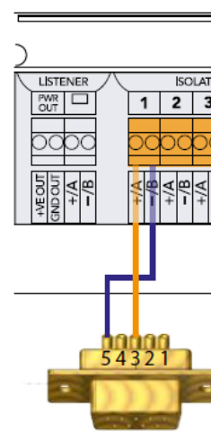
Figure 9 - RS232 Listener Connection (null modem cable)
