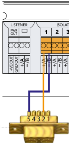
Figure 8 - RS232 Listener Connection (straight-through/extension cable)
