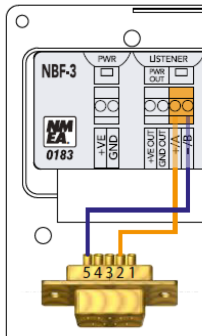
Figure 6 - RS232 Talker Connection (null modem cable)
