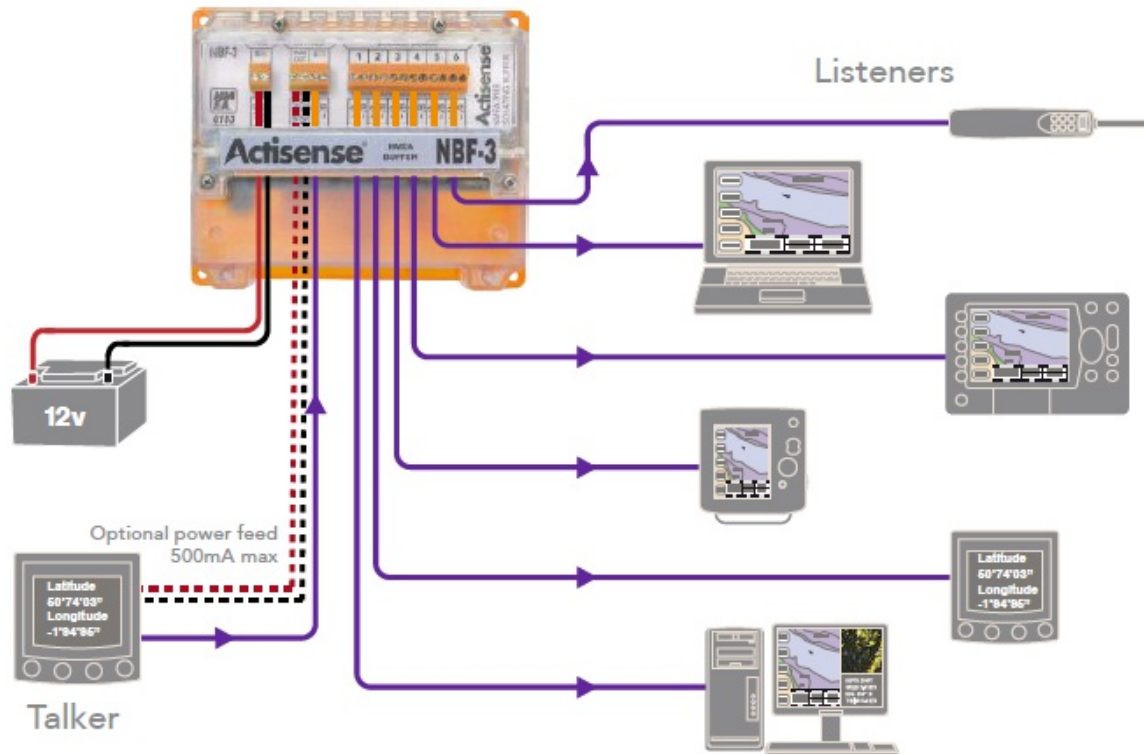
Figure 1 - Example of a Typical NBF-3 Installation
