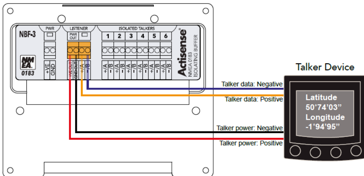
Figure 4 - Listener Port Wiring Diagram
