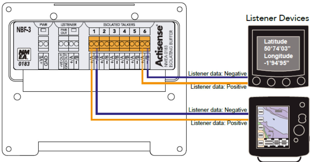
Figure 7 - Talker Port Wiring Diagram
