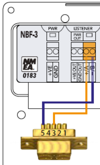
Figure 5 - RS232 Talker Connection (straight-through/extension cable)
