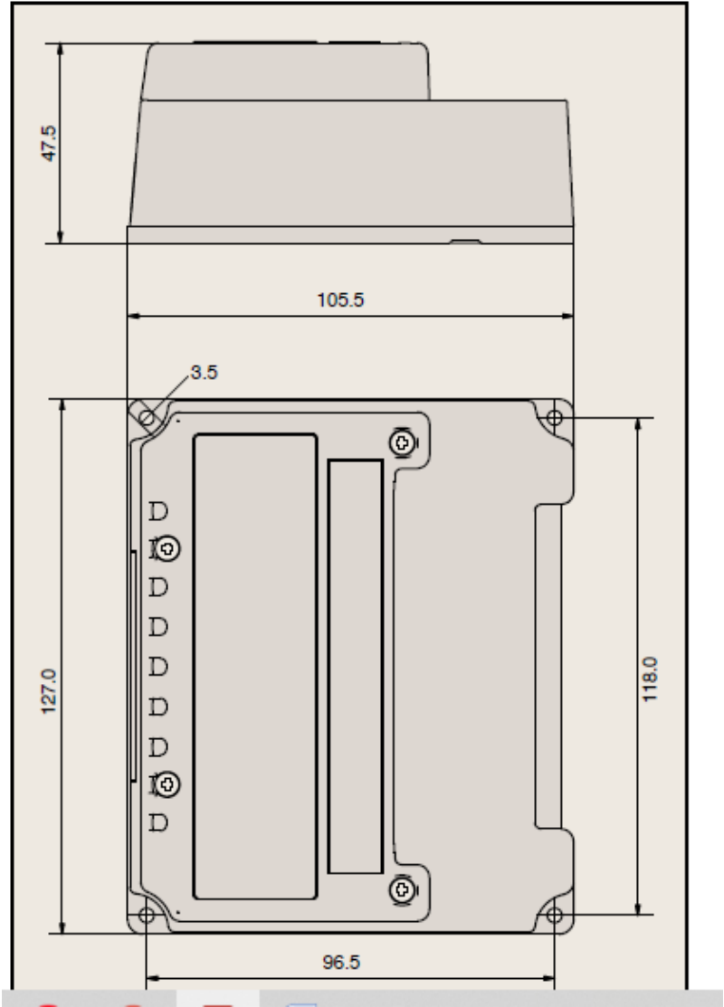
Figure 10 - Dimension Diagram
