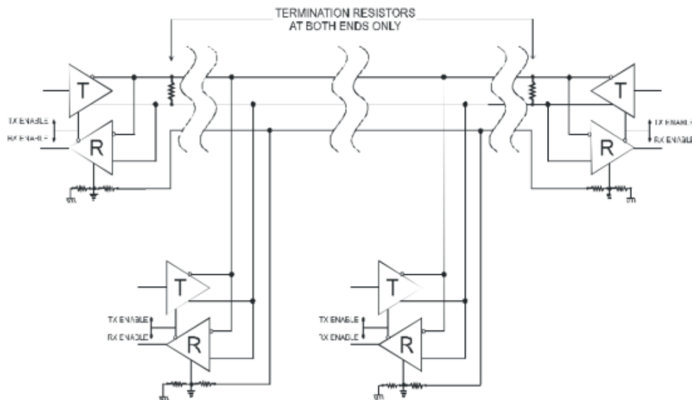
Figure A-1: Typical RS485 Two-Wire Multidrop Network
