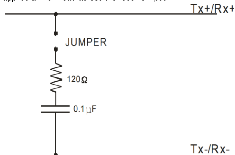
Figure 3-1: Simplified Termination Schematic
