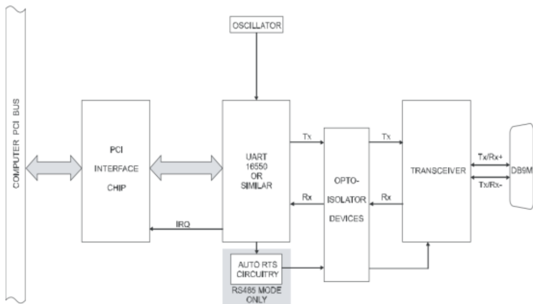
Figure 1-1: Block Diagram
