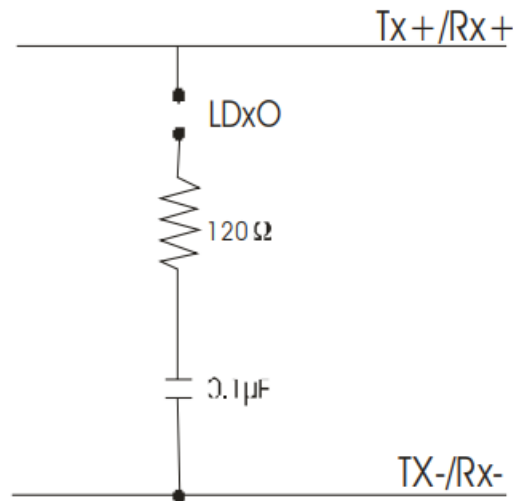
Figure 3-1: Simplified Termination Schematic
