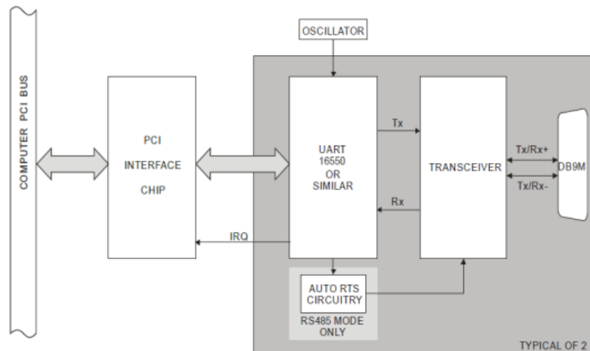
Figure 1-1: Block Diagram
