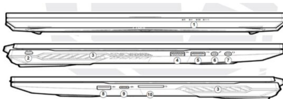
Figure 4 - Front, Left & Right Views [Model A]
