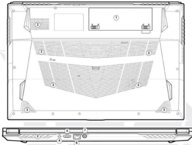
Figure 5 - Bottom & Rear Views
