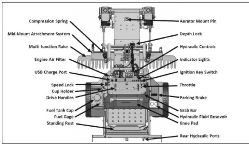
Figure 6: Control layout
