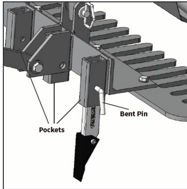
Figure 8: Scarifier installation
