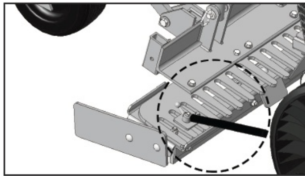
Figure 9: Mini-box clamp rotate
