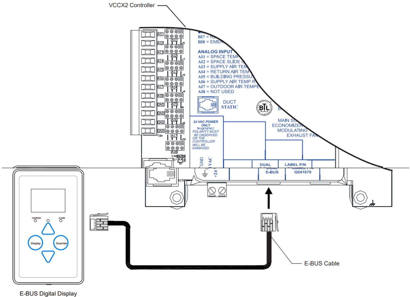
Figure 3: E-BUS Digital Display Wiring to Controller
