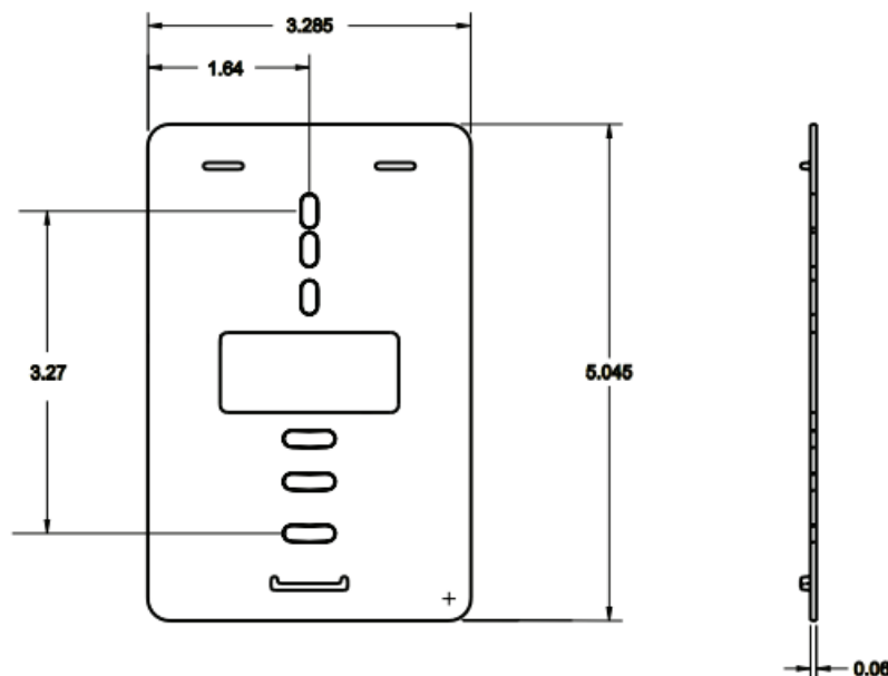
Figure 14: Mounting Plate Dimensions
