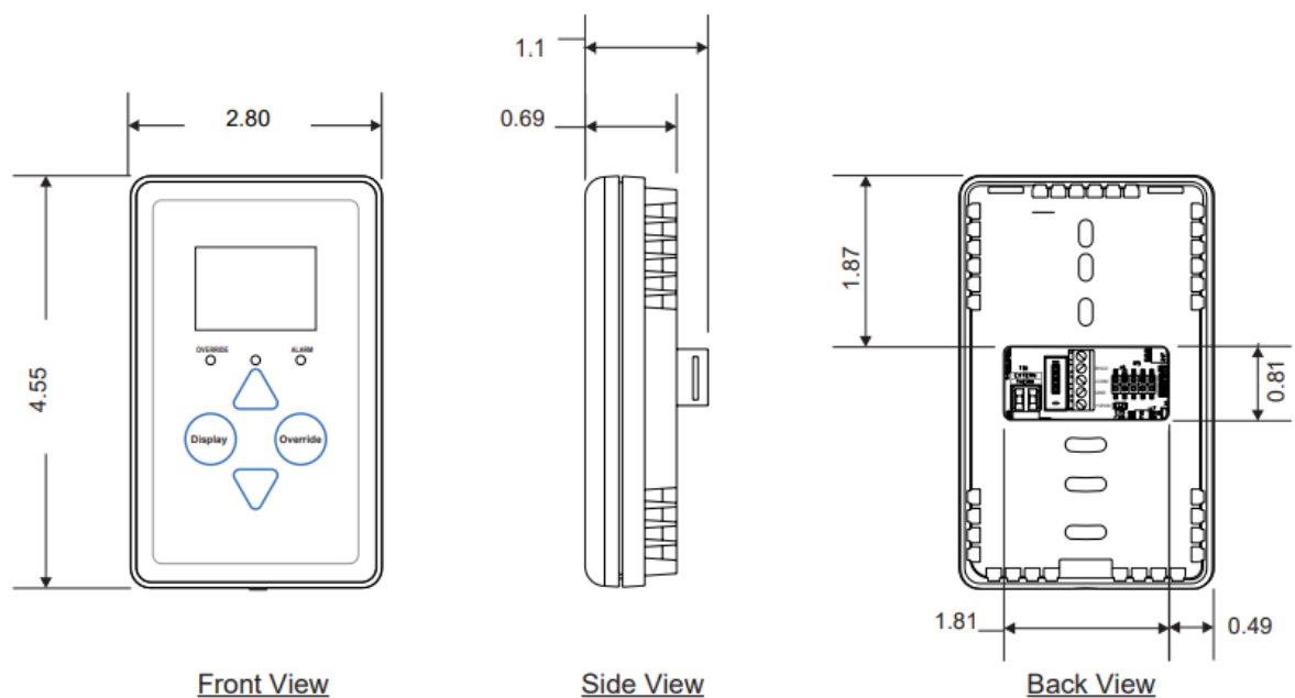
Figure 2: Dimensions
