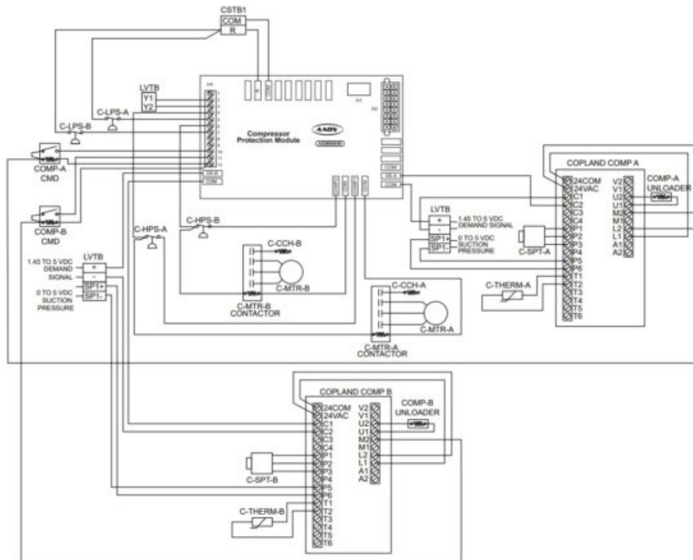
Figure 7: ASM06690 – Dual Digital Compressors
