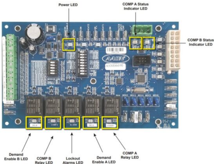
Figure 14: LED Locations and Descriptions – ASM06690
