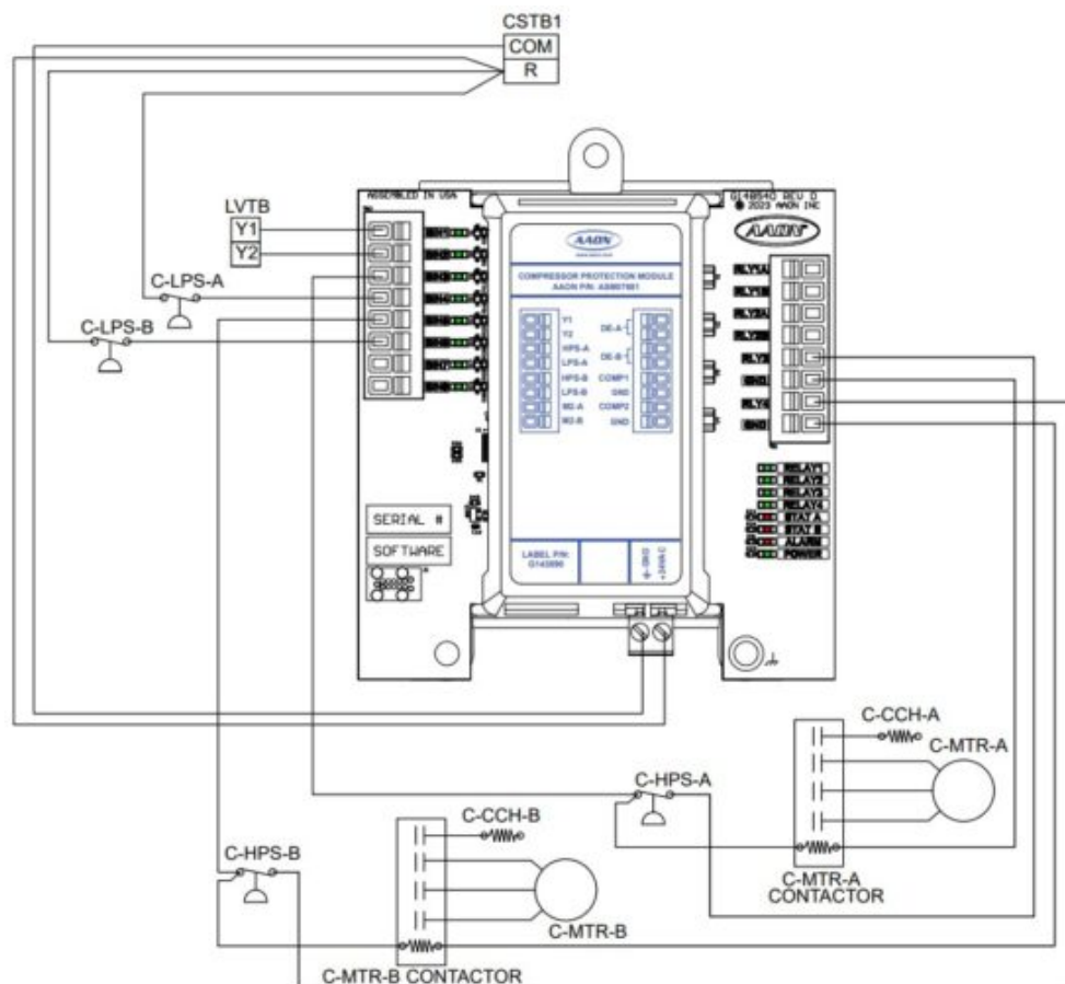
Figure 9: ASM07681 – Dual Compressor
