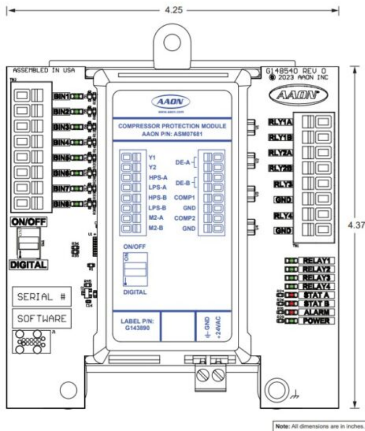
Figure 2: Compressor Protection Module Dimensions – ASM07681
