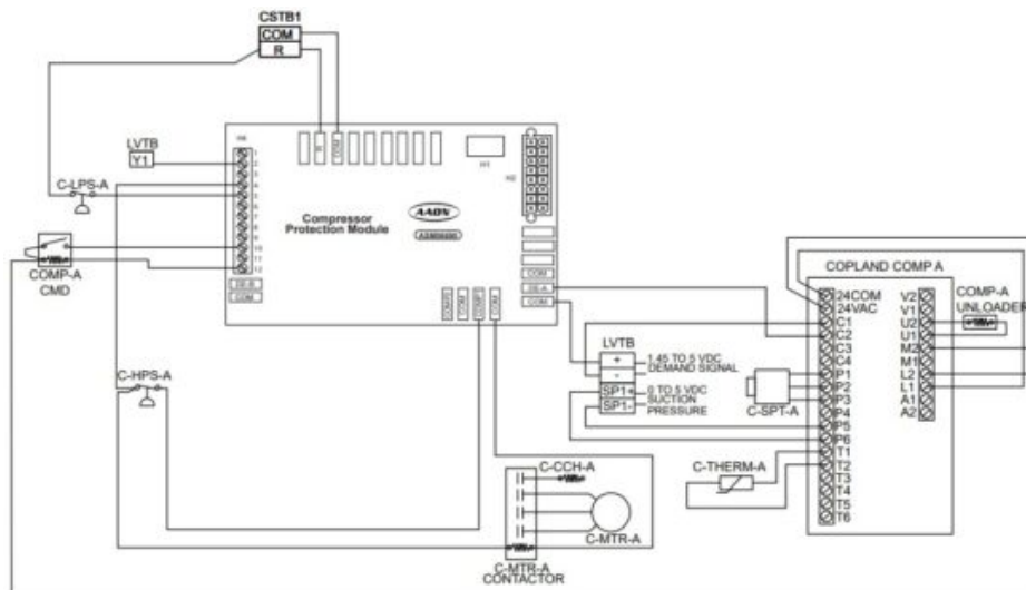
Figure 5: ASM06690 – Single Digital Compressor
