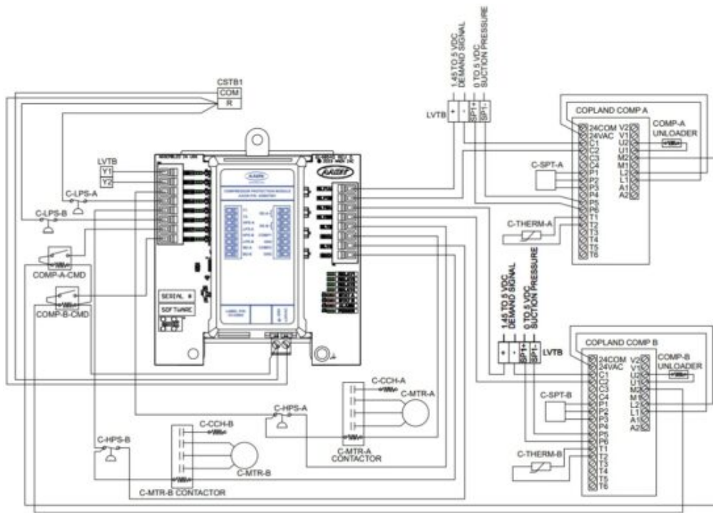
Figure 12: ASM07681 – Dual Digital Compressors
