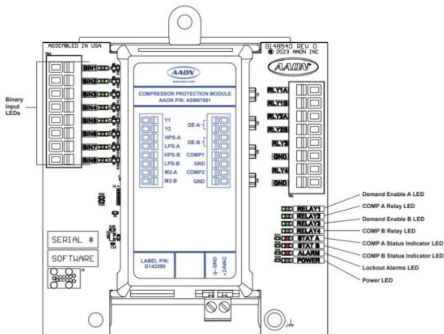
Figure 15: LED Locations and Descriptions – ASM07681
