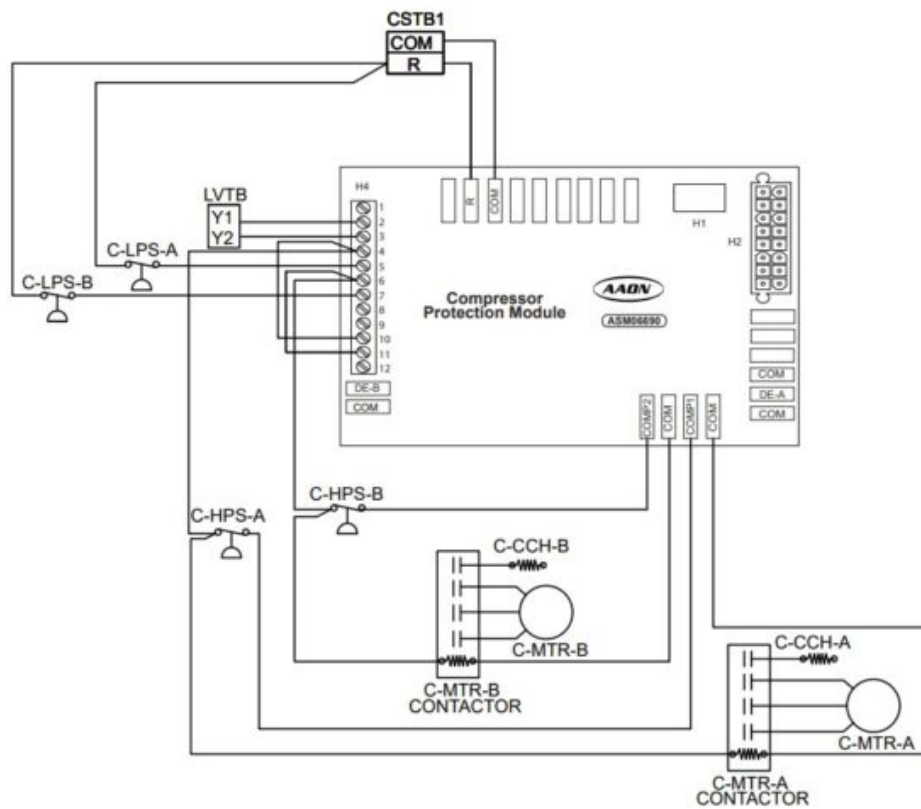
Figure 4: ASM06690 – Dual Compressor
