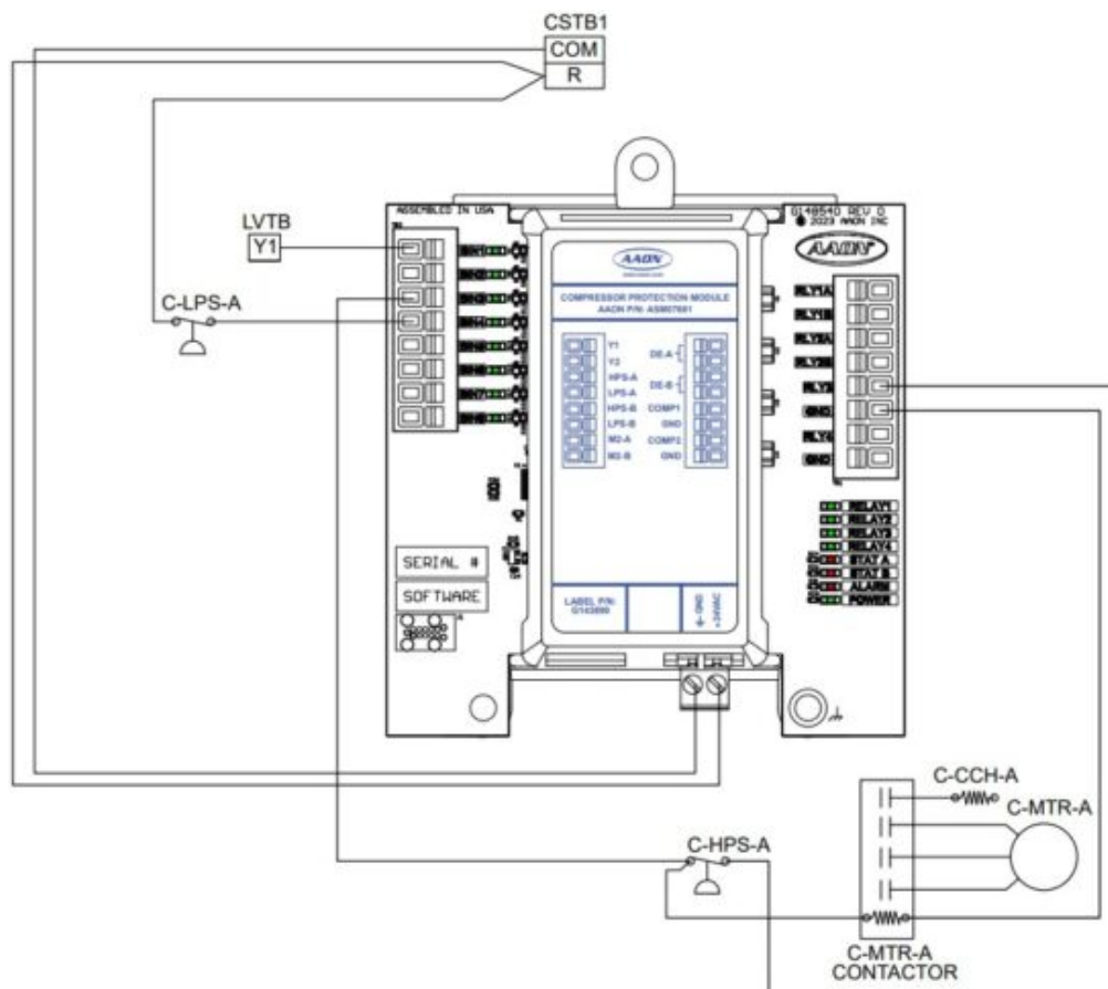
Figure 8: ASM07681 – Single Compressor
