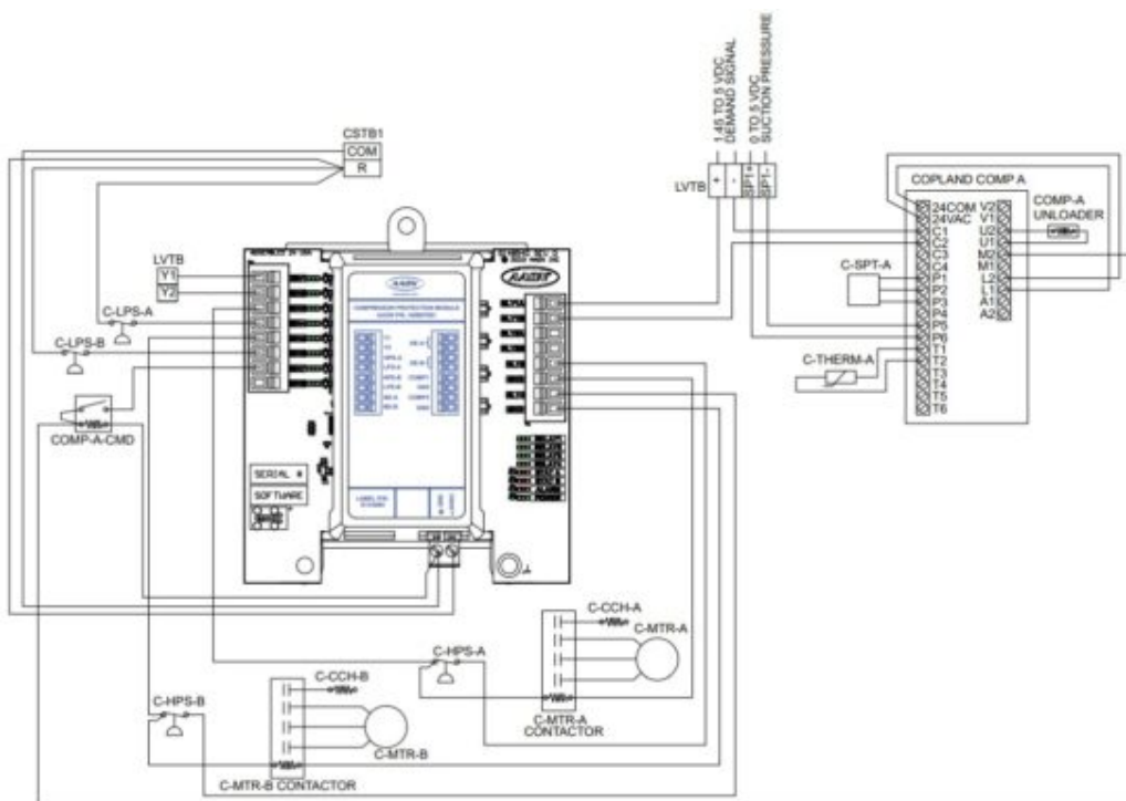
Figure 11: ASM07681 – Digital and On/Off Compressor
