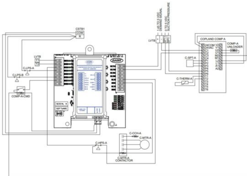
Figure 10: ASM07681 – Single Digital Compressor
