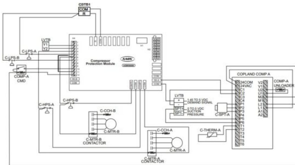
Figure 6: ASM06690 – Digital and On/Off Compressor
