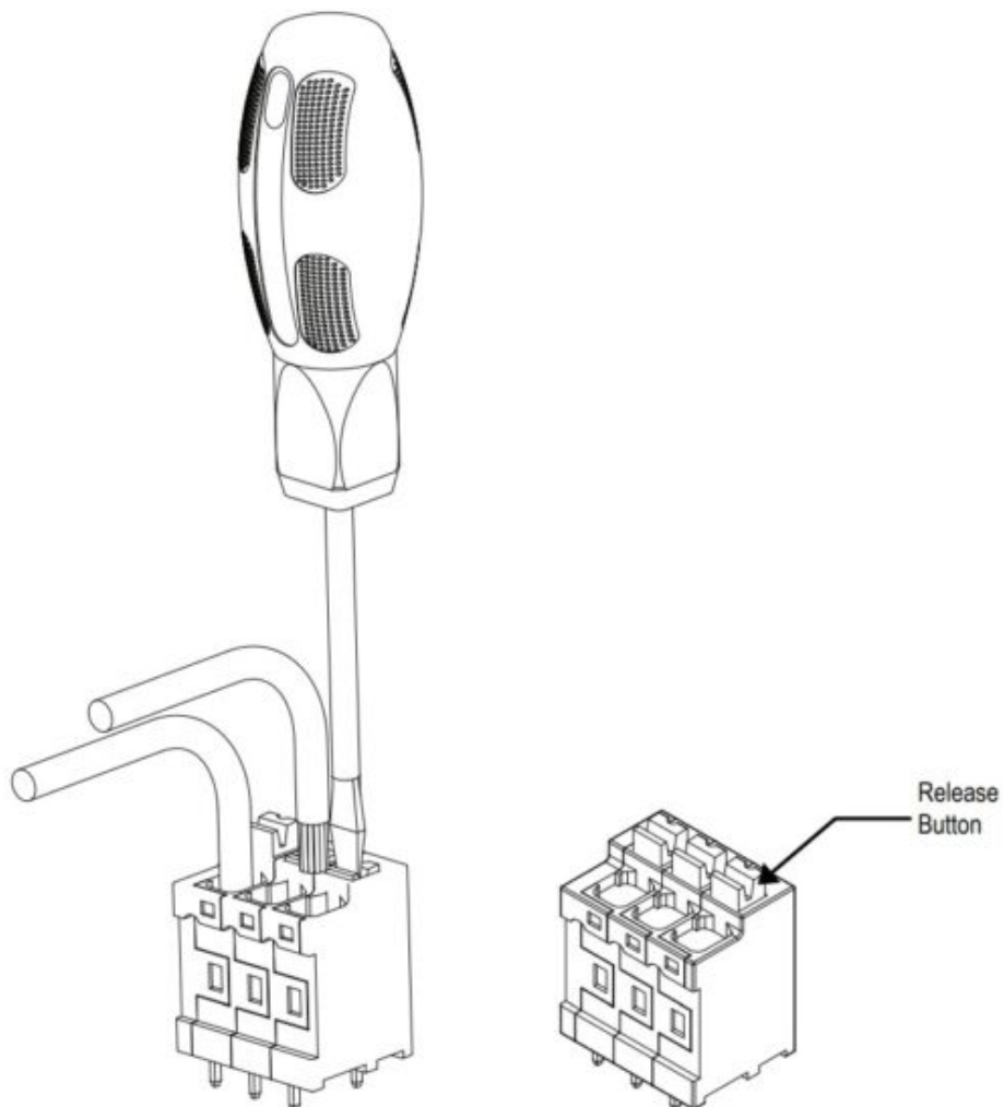
Figure 13: OMNIMATE Connector Instructions
