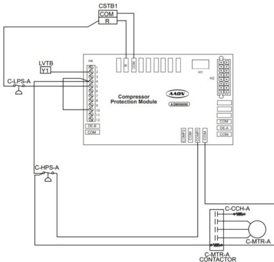
Figure 3: ASM06690 – Single Compressor
