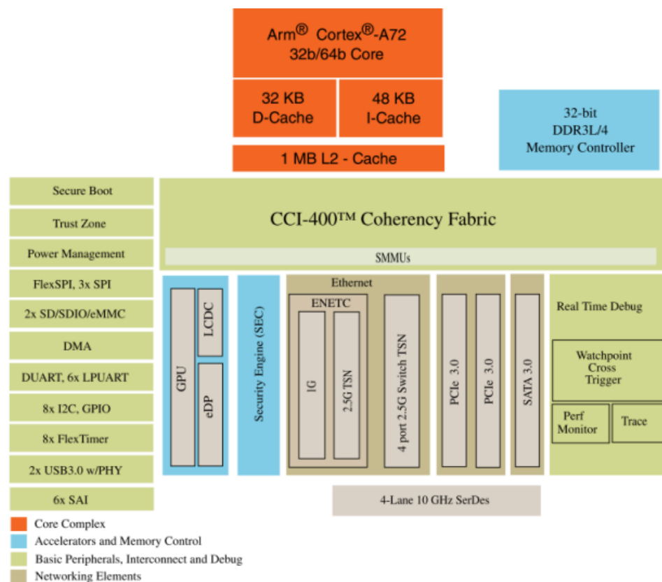
Figure 2: Block diagram LS1028A (Source: NXP )
