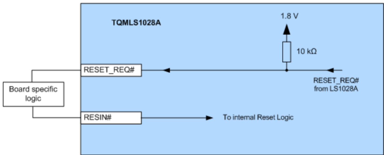
Figure 7: Block diagram RESET_REQ# / RESIN# TQMLS1028A revision 01xx
