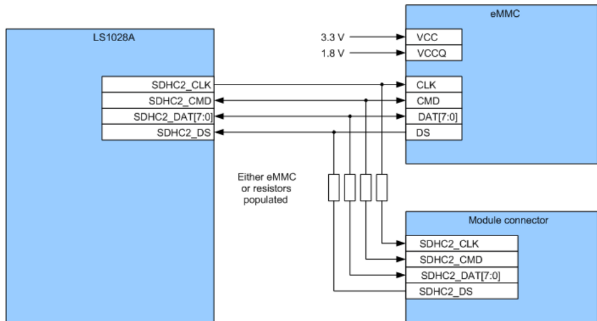
Figure 9: Block diagram eMMC interface
