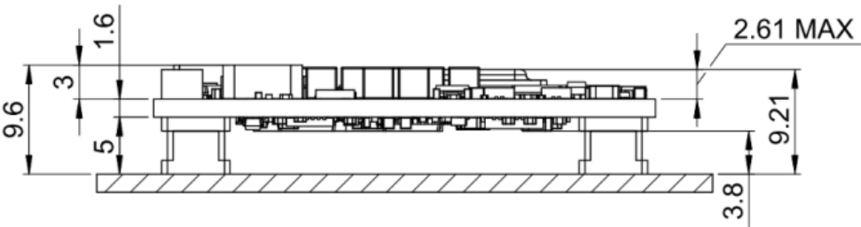
Figure 18: TQMLS1028A dimensions, side view
