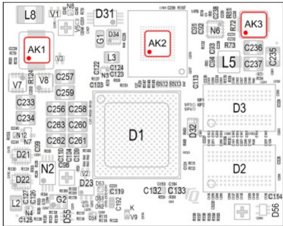
Figure 14: TQMLS1028A assembly revision 01xx, top
