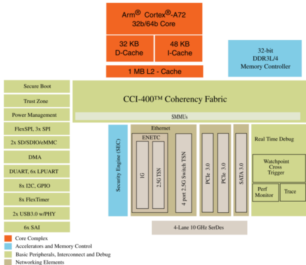
Figure 5: Block diagram LS1017A (Source: NXP )
