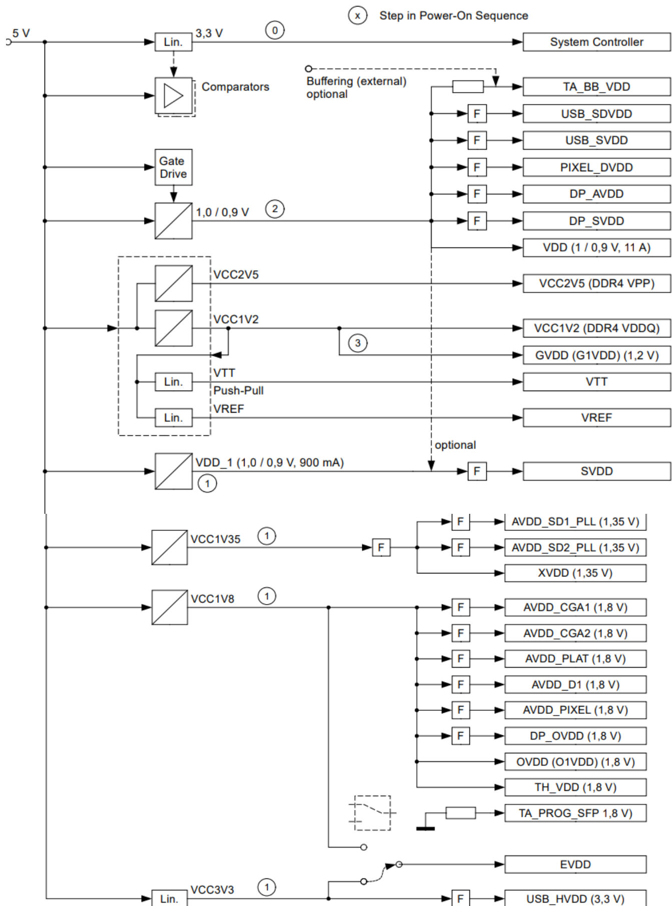
Figure 12: Module supply overview
