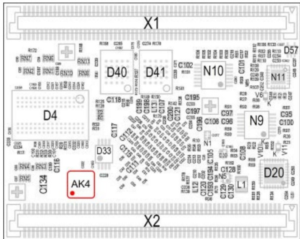
Figure 15: TQMLS1028A assembly revision 01xx, bottom
