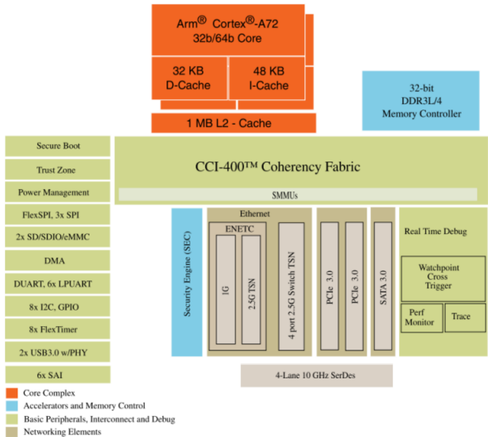
Figure 4: Block diagram LS1027A (Source: NXP )
