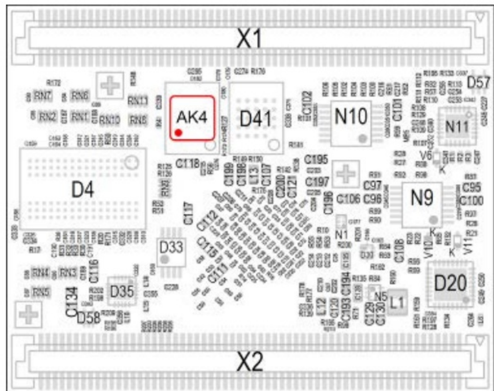
Figure 17: TQMLS1028A assembly revision 02xx, bottom
