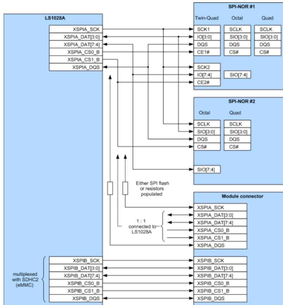
Figure 8: Block diagram QSPI interface
