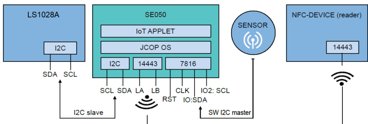
Figure 13: Block diagram SE050 (Source: NXP )
