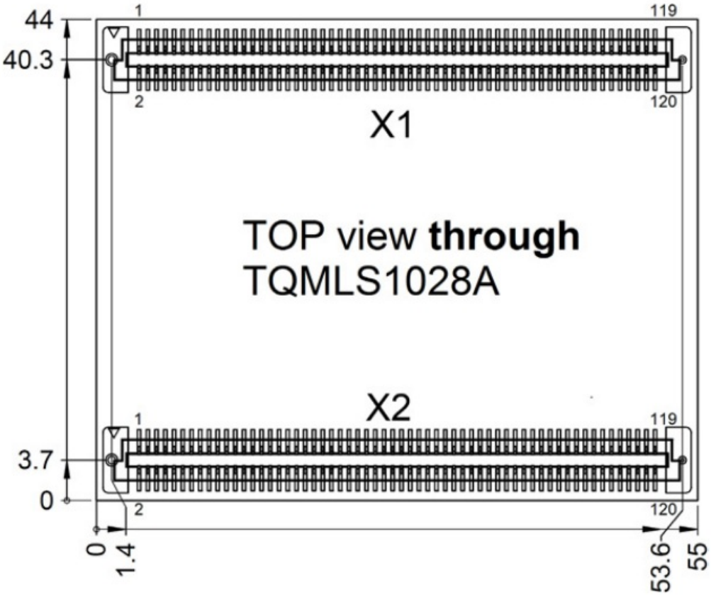
Figure 19: TQMLS1028A dimensions, top view through TQMLS1028A
