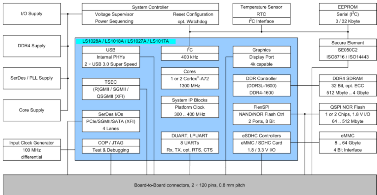
Figure 1: Block diagram TQMLS1028A (simplified)
