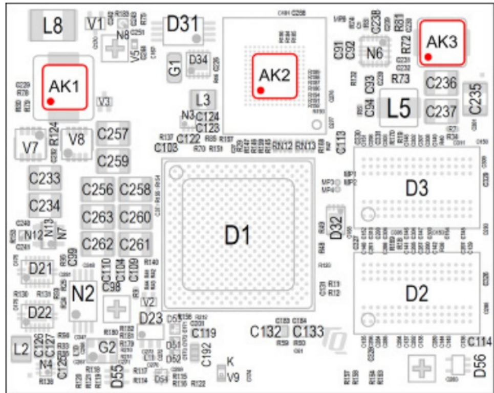
Figure 16: TQMLS1028A assembly revision 02xx, top
