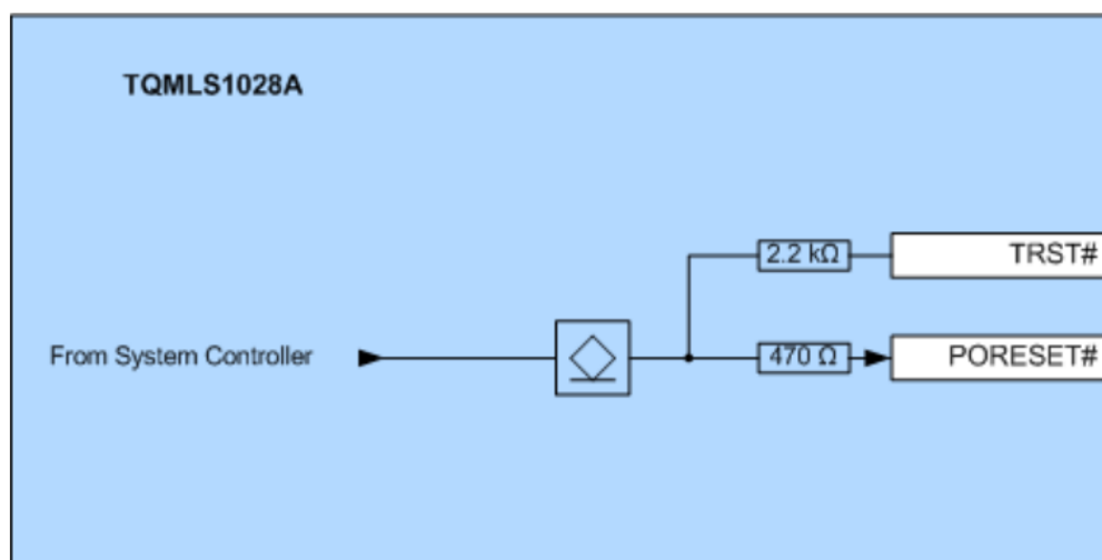
Figure 6: Block diagram TRST#
