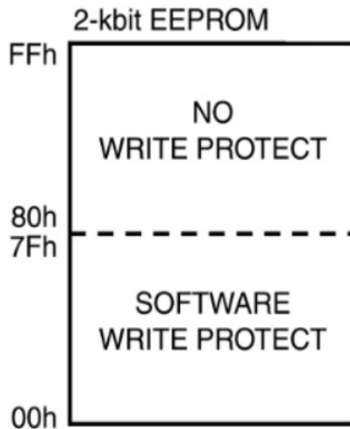
Figure 10: Memory Map SE97BTP EEPROM
