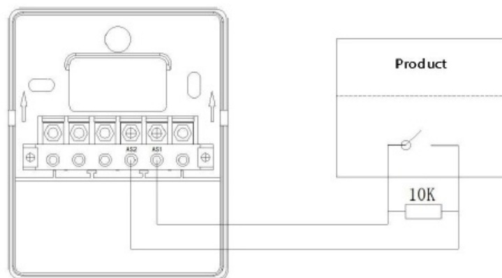
Fig.4 Wiring diagram
