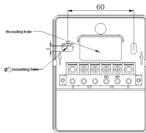
Fig.2 Installation method
