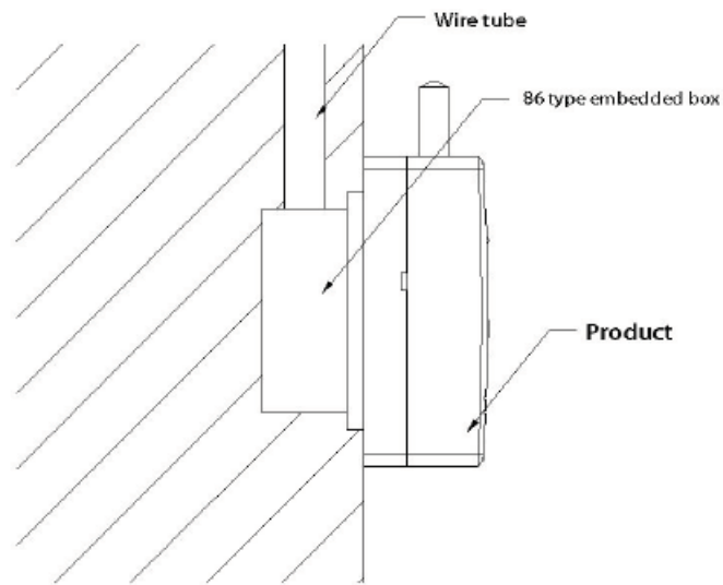
Fig.2 Installation method
