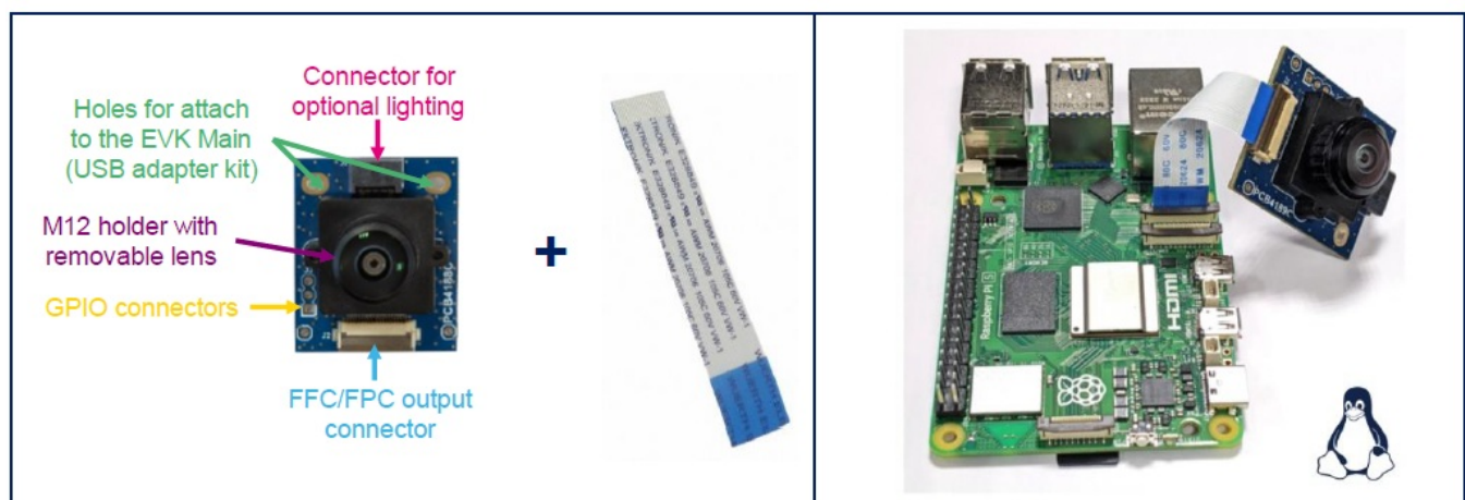
Figure 2. Illustration of S-Board content and associated setup
