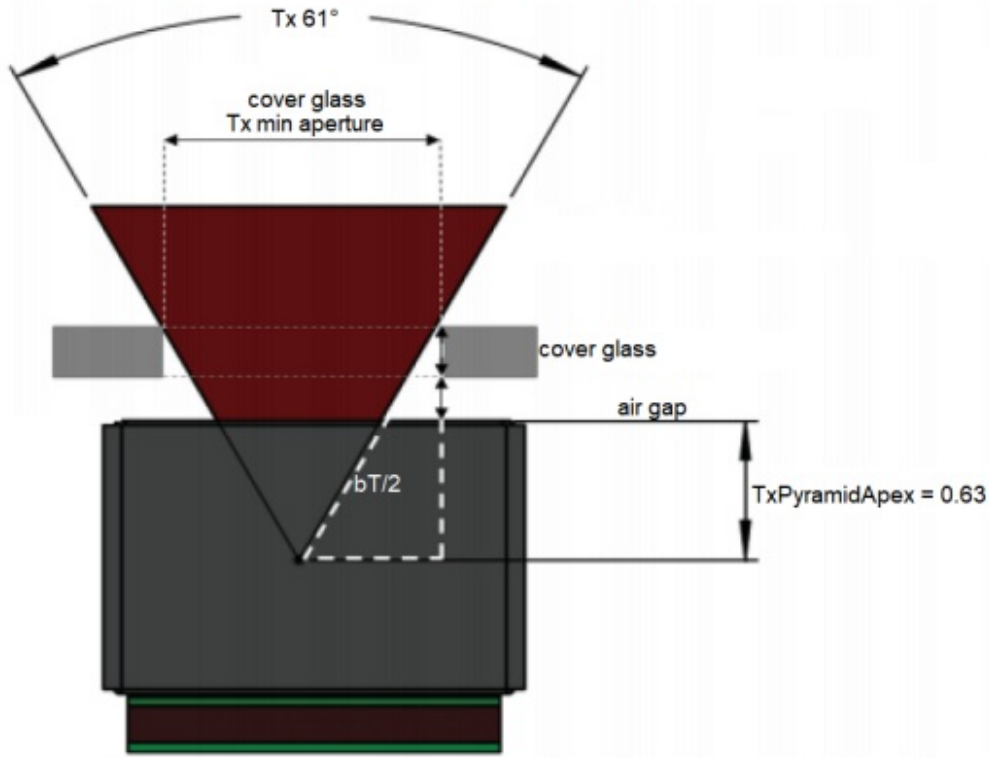
Figure 9. Cover glass Tx aperture in y direction
