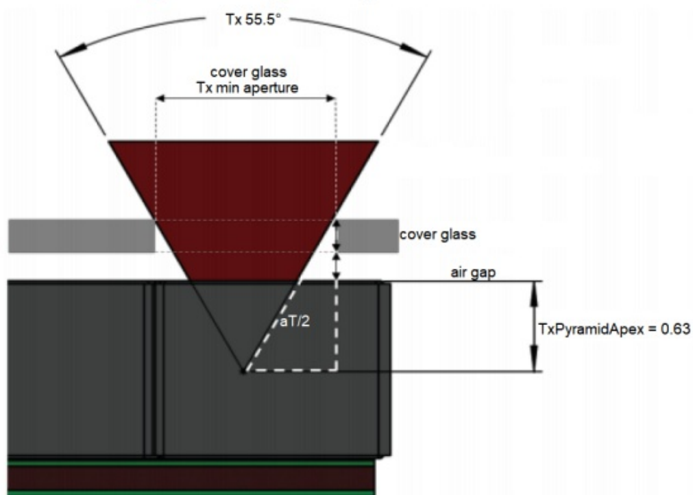
Figure 8. Cover glass Tx aperture in x direction
