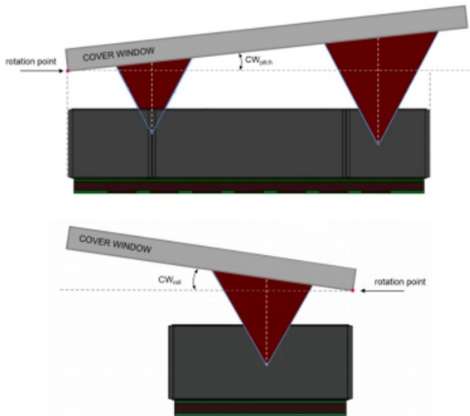
Figure 13. Aperture shapes with cover glass rotation
