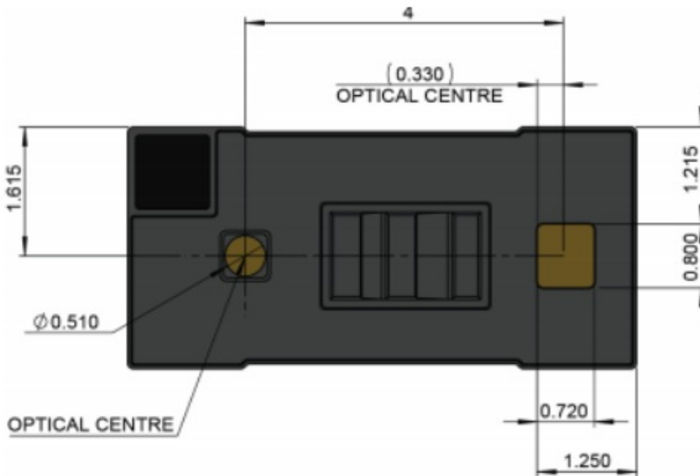
Figure 6. VL53L5CX mechanical dimensions
