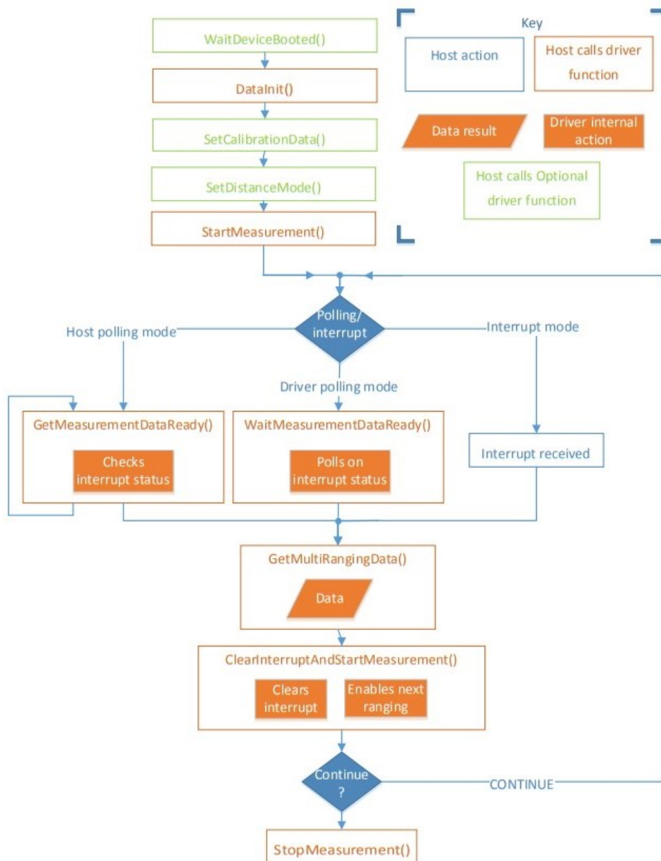
Figure 5. VL53L3CX API ranging flow (field)
