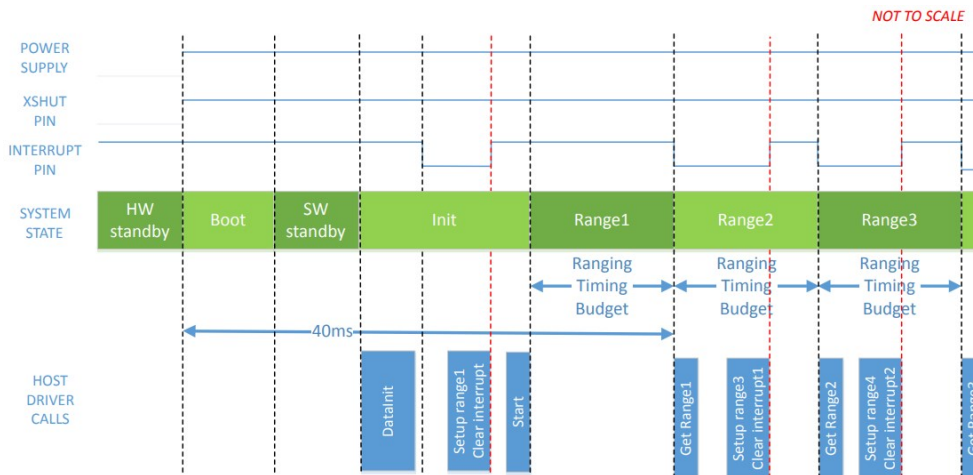
Figure 3. Ranging sequence and timing targets
