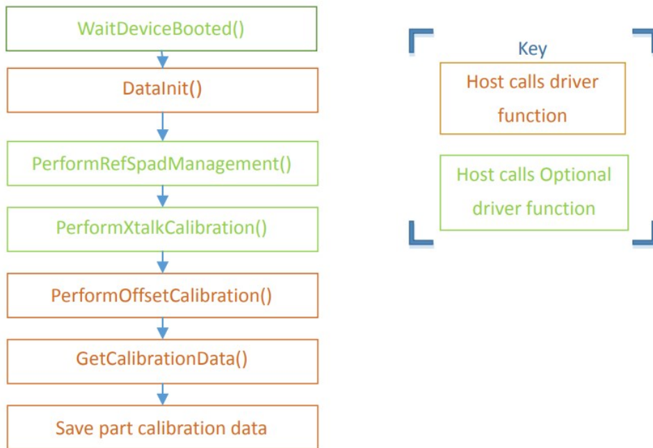
Figure 4. VL53L3CX API ranging flow (factory)
