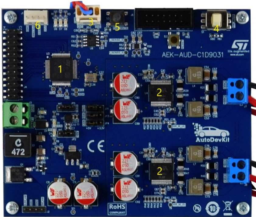
Figure 3. AEK-AUD-C1D9031 components
