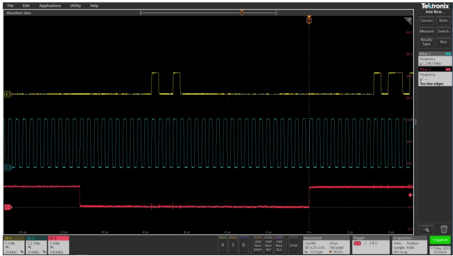
Figure 12. I 2 S simulated signal (zoom)
