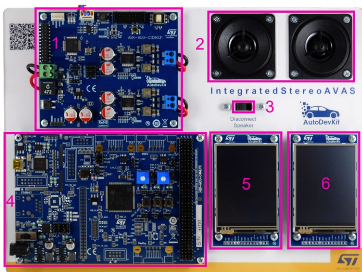
Figure 2. Kit components
