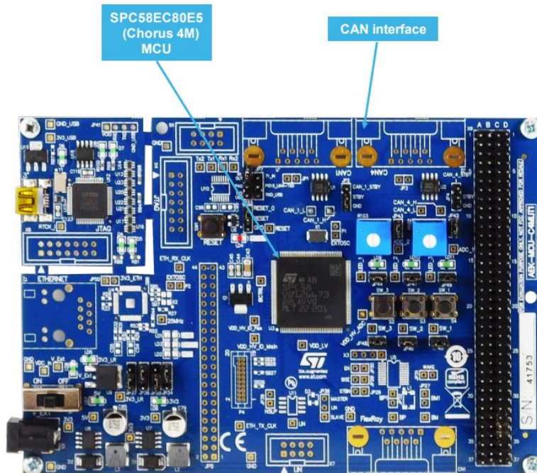
Figure 4. AEK-MCU-C4M1LIT1 MCU board
