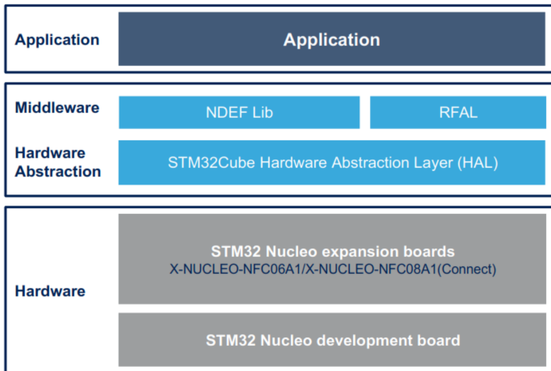
Figure 2. X-CUBE-NFC6 software architecture
