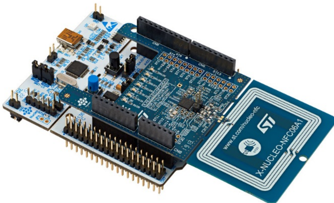
Figure 11. X-NUCLEO-NFC06A1 expansion board plus NUCLEO-L476RG development board
