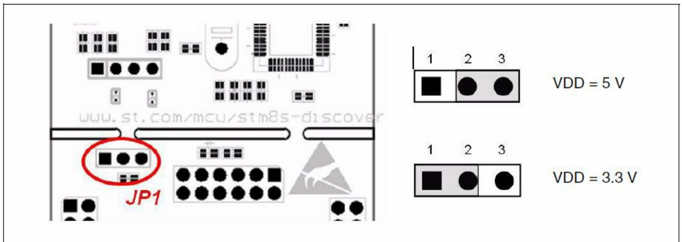
Figure 9. Power selection
