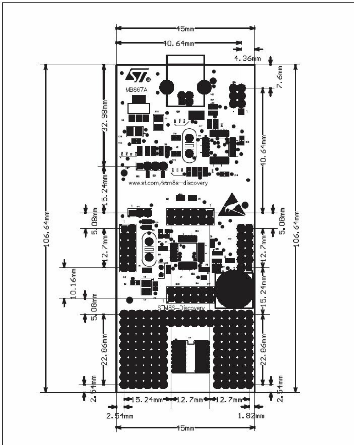
Figure 11. STM8S-DISCOVERY
