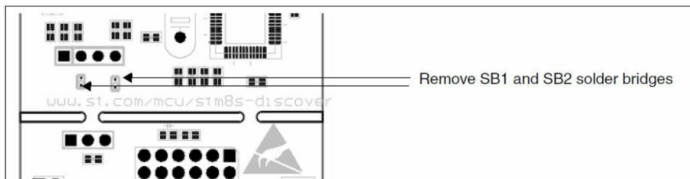
Figure 8. Separated ST-LINK module
