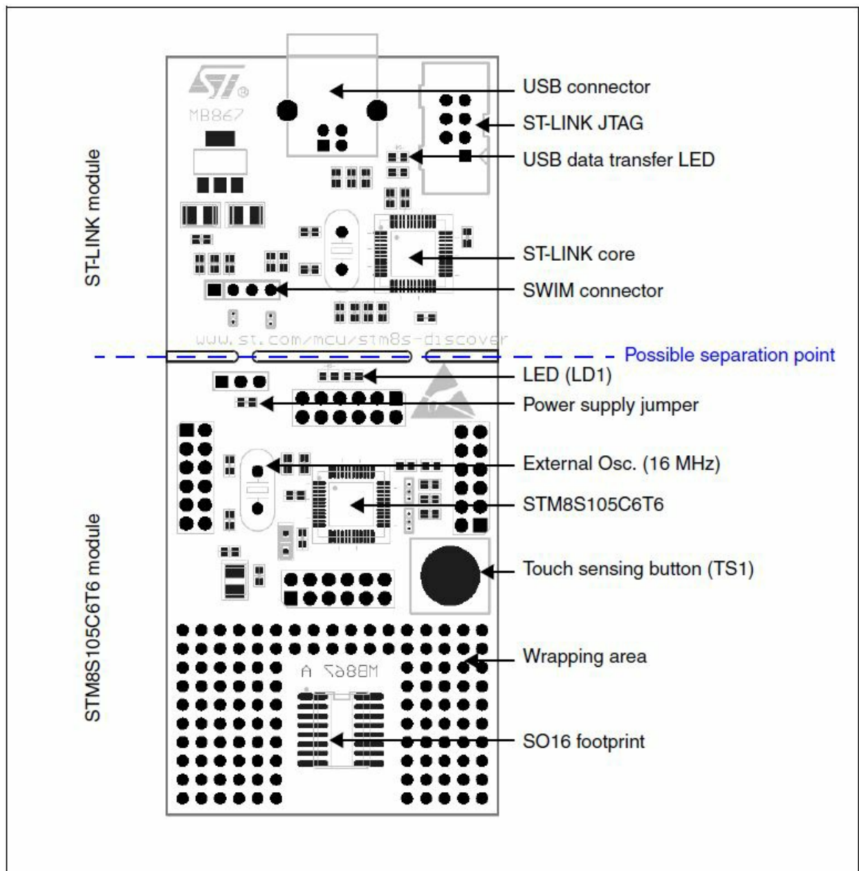
Figure 4. STM8S105C6T6 package
