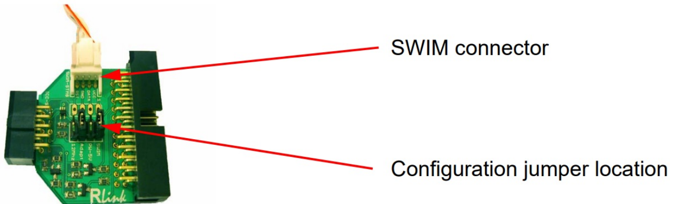
Figure 9. RLink USB and SWIM configuration
