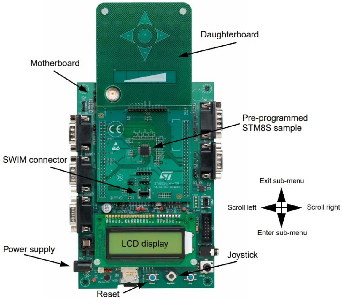
Figure 2. TS evaluation kit assembly
