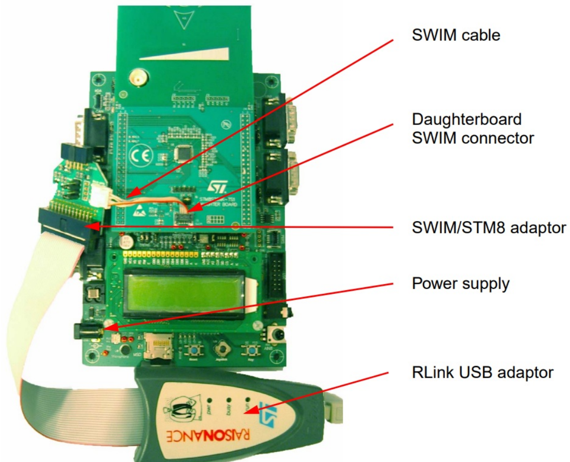
Figure 9. RLink USB and SWIM configuration
