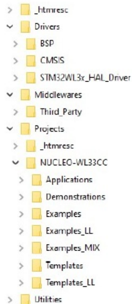
Figure 3. STM32CubeWL3 firmware package structure
