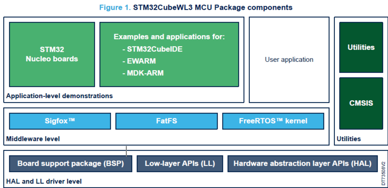
Figure 1. STM32CubeWL3 MCU Package components
