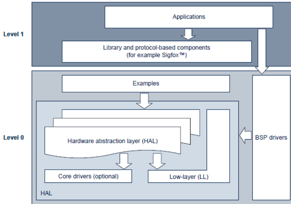
Figure 2. STM32CubeWL3 MCU Package architecture
