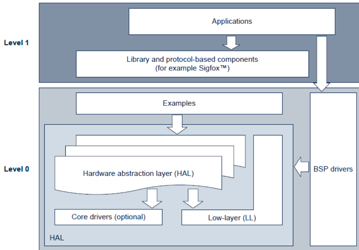
Figure 2. STM32CubeWL3 MCU Package architecture
