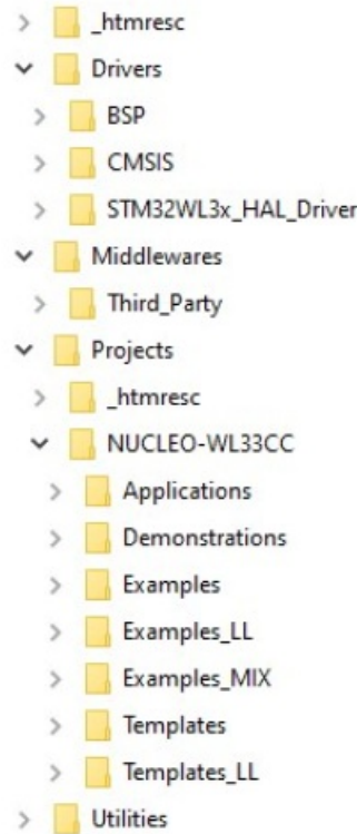
Figure 3. STM32CubeWL3 firmware package structure
