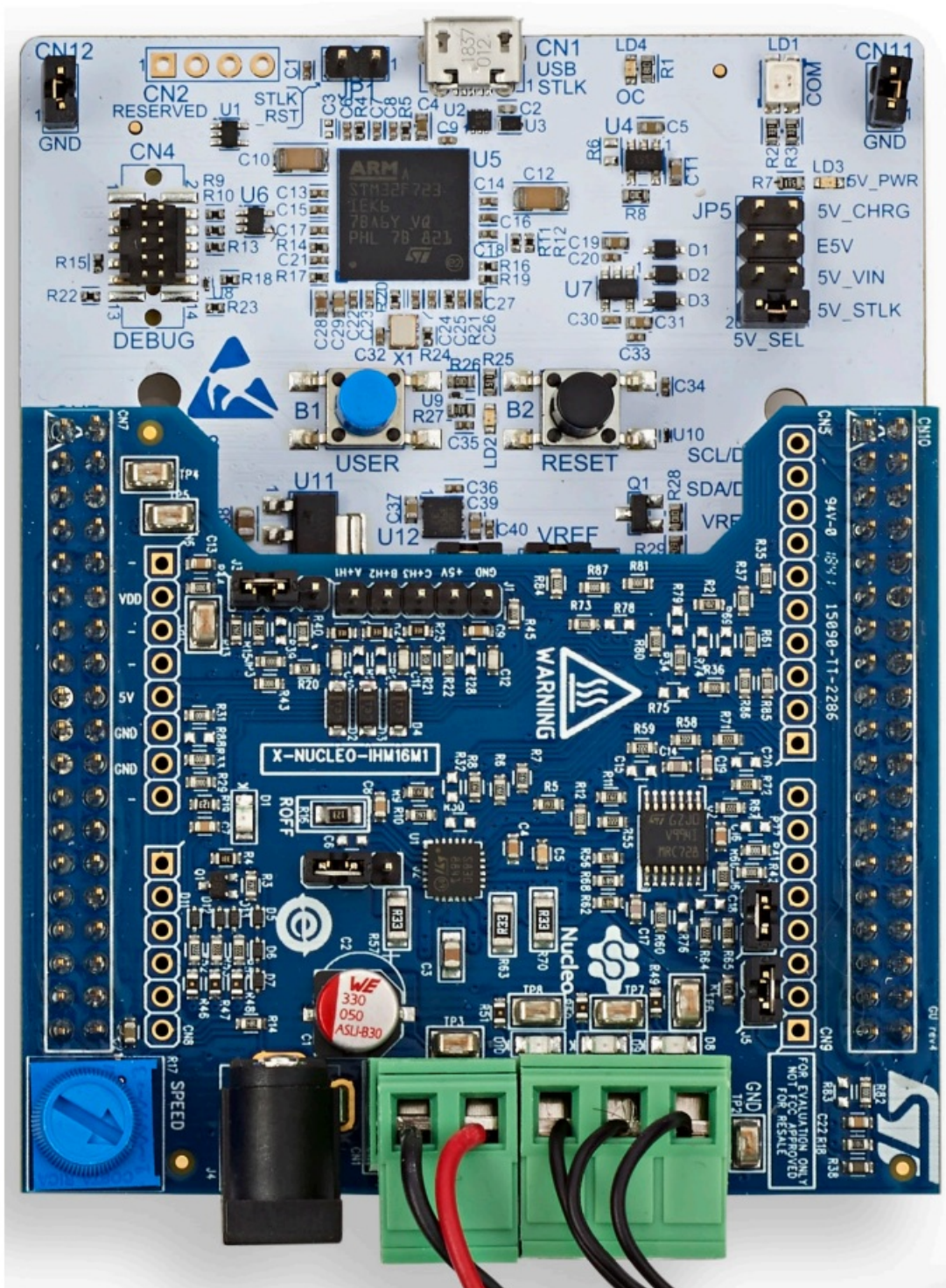
Figure 3. X-NUCLEO-IHM16M1 and NUCLEO-G431RB assembled
