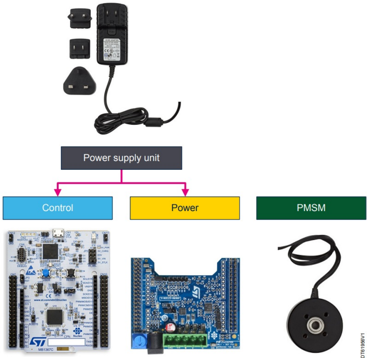
Figure 2. Four-block architecture of the P-NUCLEO-IHM03 pack
