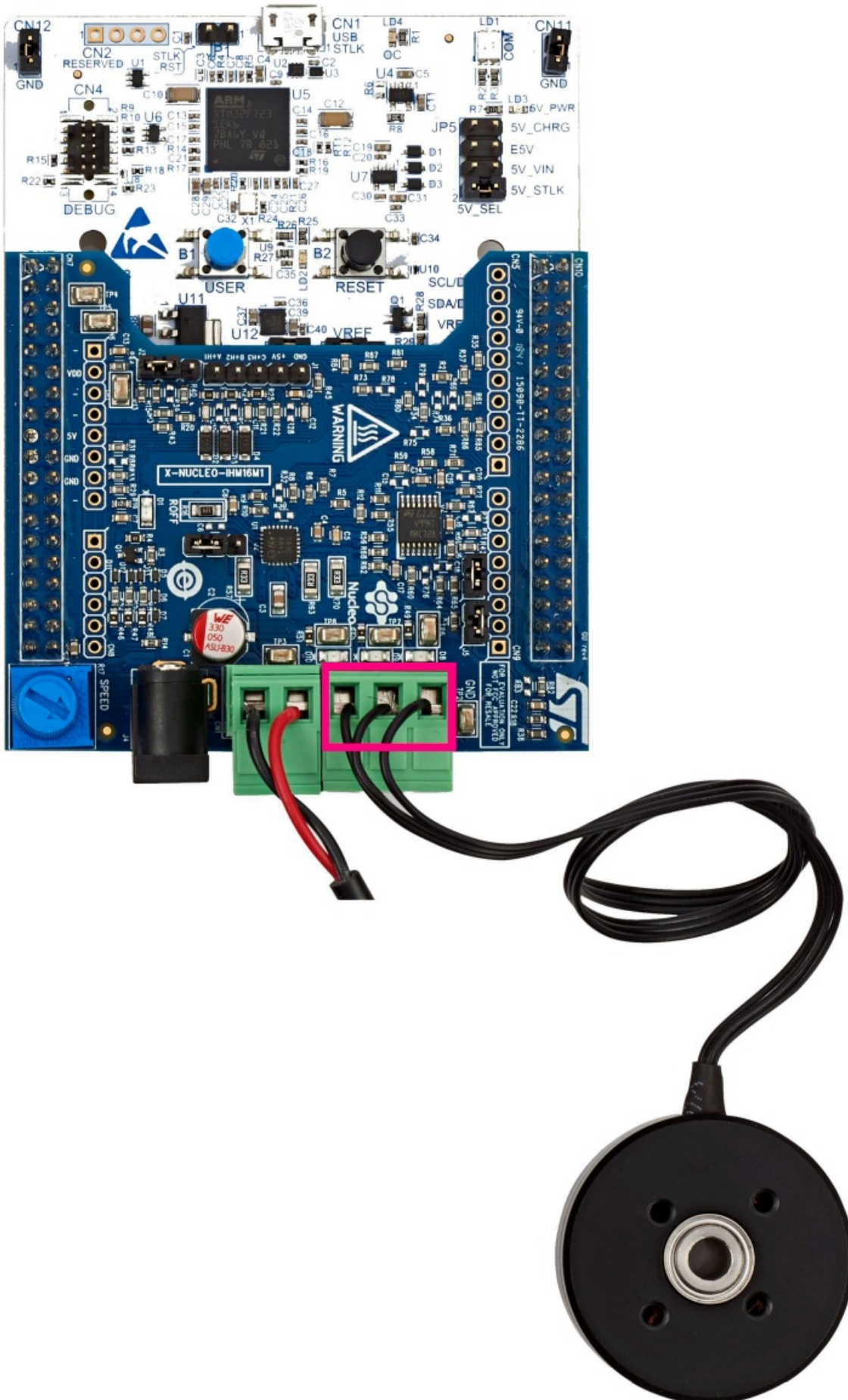
Figure 4. Motor connection with X-NUCLEO-IHM16M1
