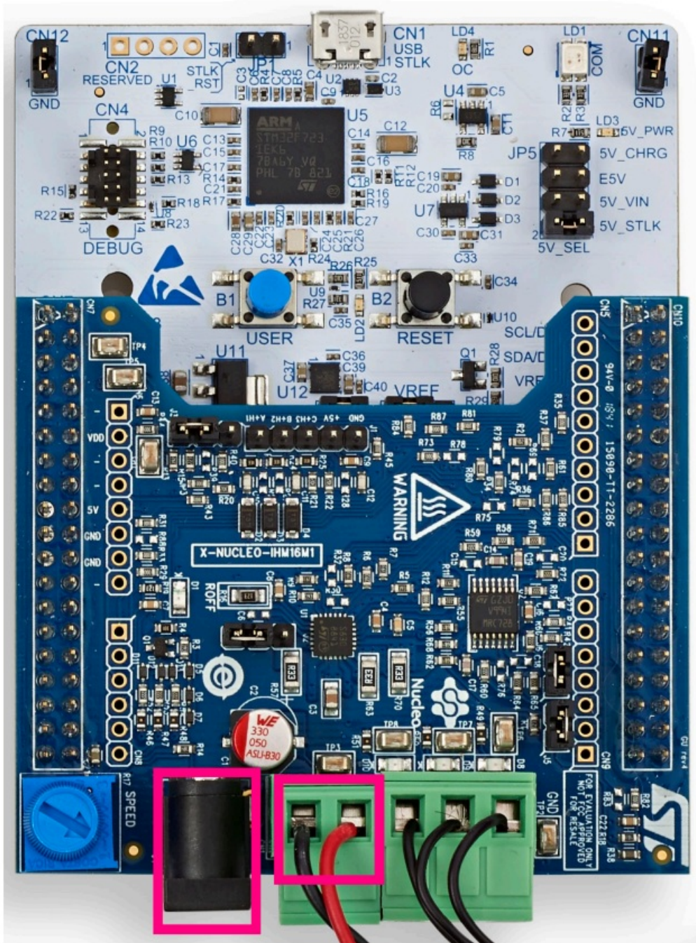
Figure 5. Power-supply connection for X-NUCLEO-IHM16M1
