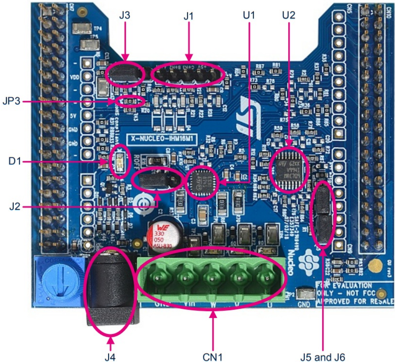
Figure 6. X-NUCLEO-IHM16M1 connectors
