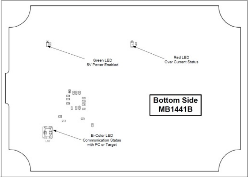
Figure 9. MB1441 bottom layout
