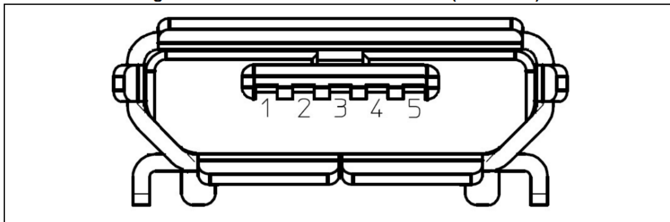
Figure 14. USB Micro-B connector CN5 (front view)
