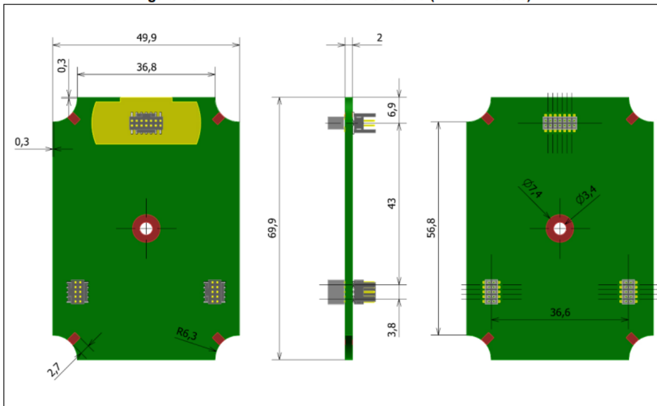
Figure 15. MB1441 mechanical dimensions (in millimeters)
