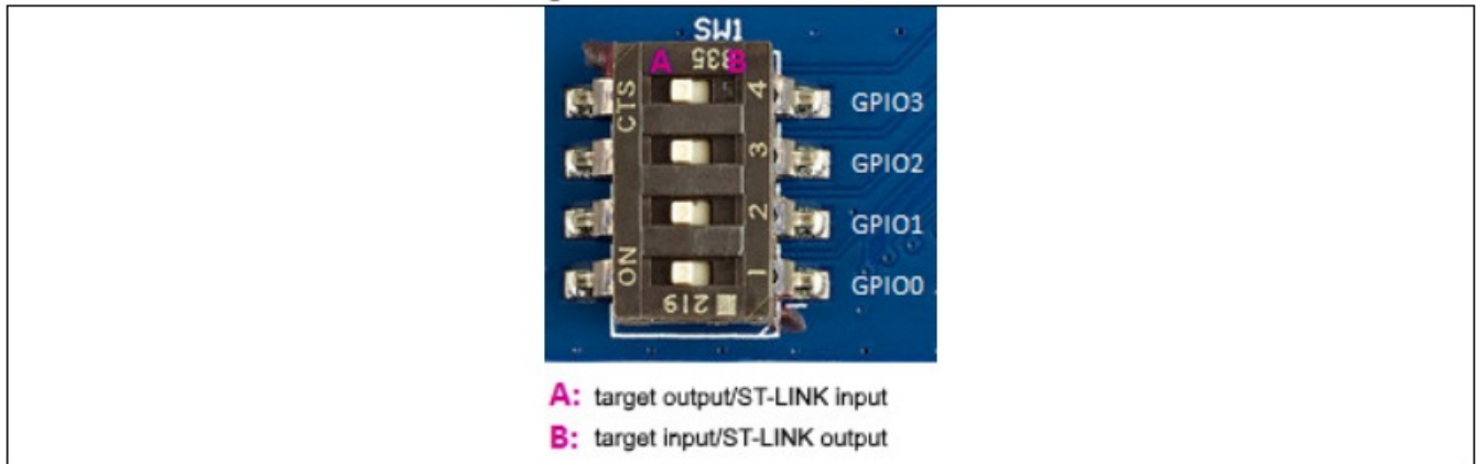
Figure 18. B-STLINK-VOLT
