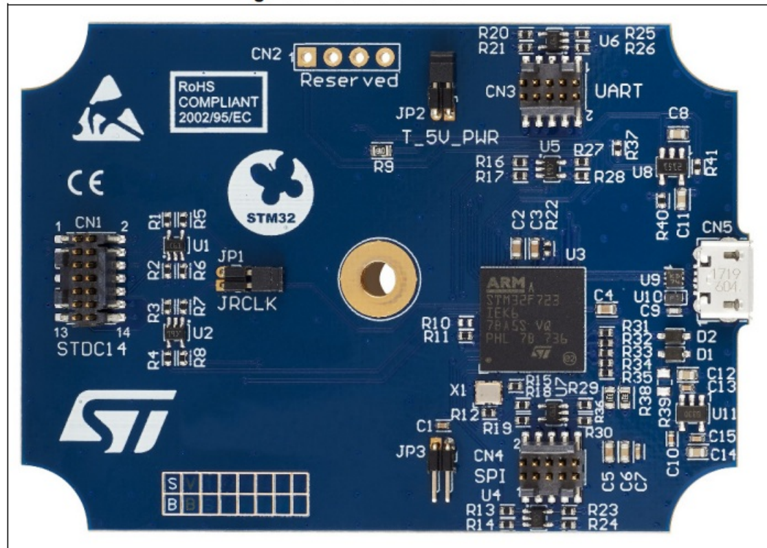
Figure 6. Hardware board MB1441
