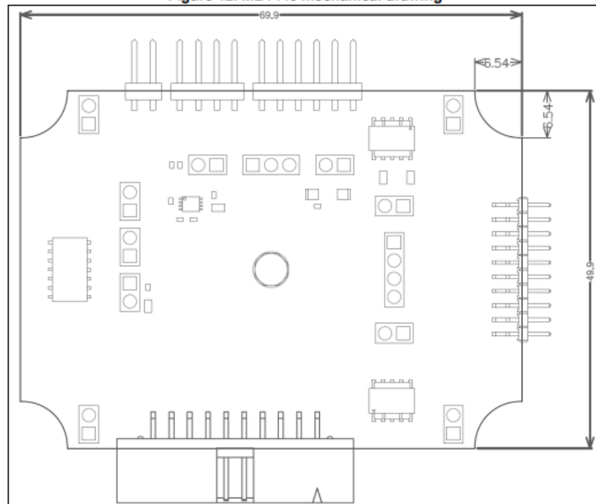
Figure 12. MB1440 mechanical drawing
