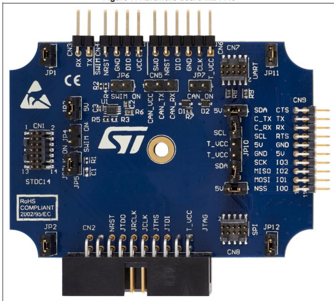
Figure 7. Hardware board MB1440
