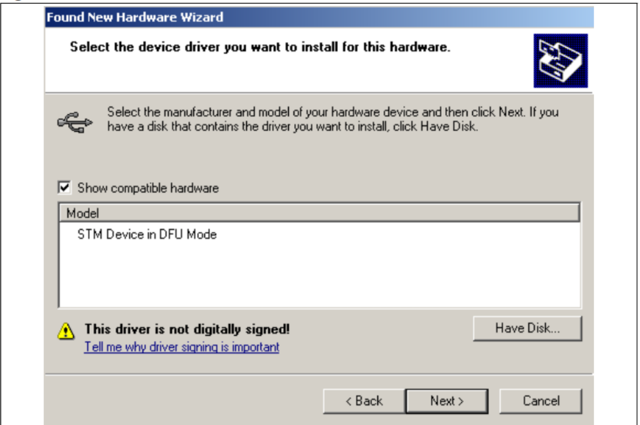
Figure 4. Driver selection
