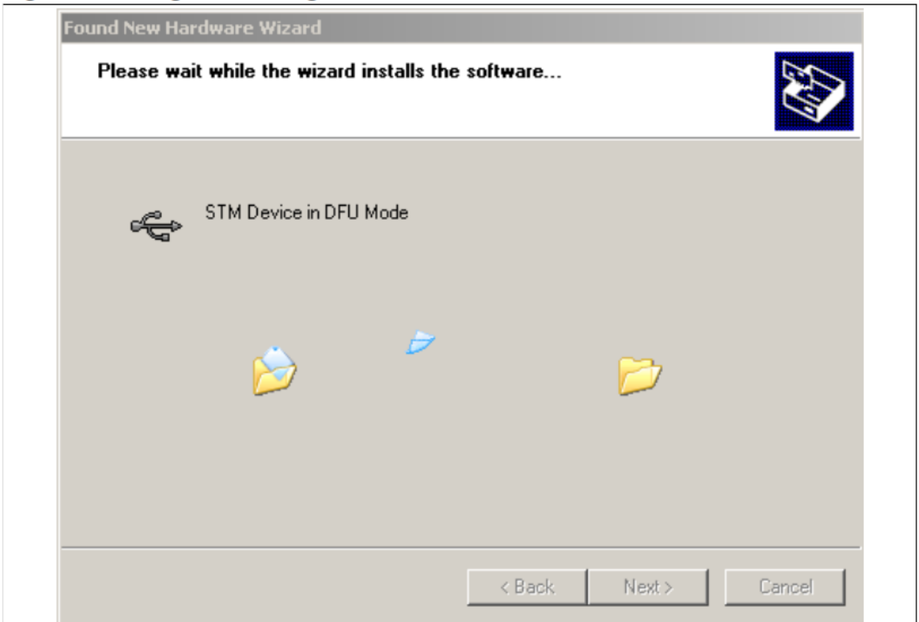
Figure 6. Progress message
