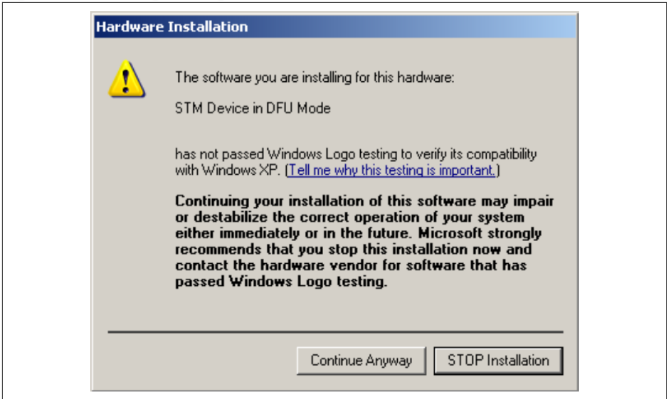
Figure 7. Warning message
