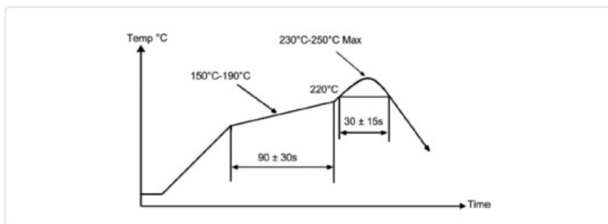
Figure 6: F1 Smart Module Recommended Reflow Soldering Profile
