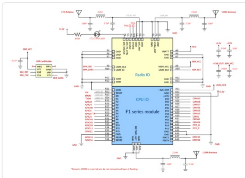
Figure 5: F1 Smart Module Recommended Basic Circuit
