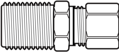
Male Straight Tube Fitting Tube fitting for 1/4" air line, with a thread size to match the street tee fitting.
