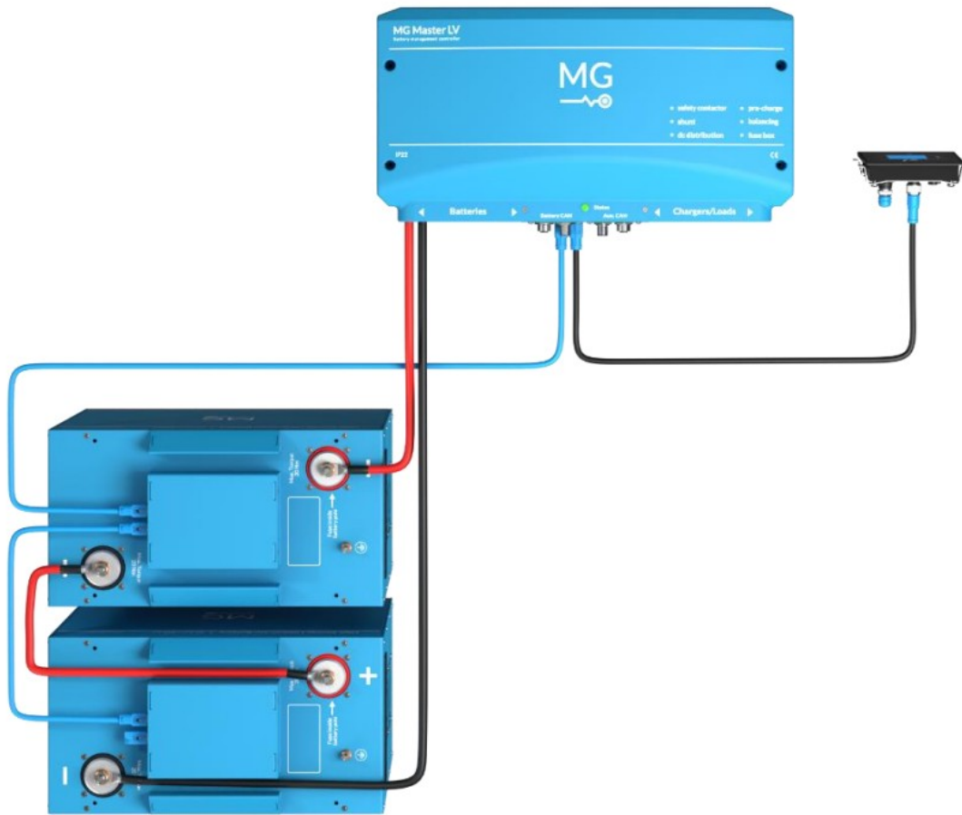
Figure 15 - Example system
