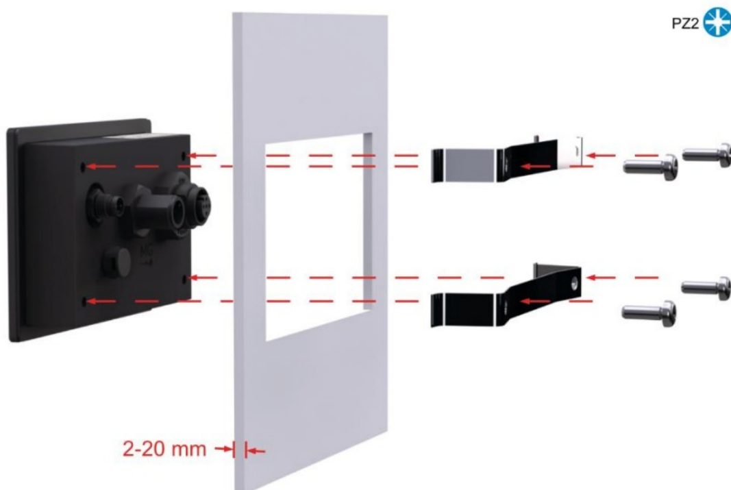
Figure 14 - Mounting procedure
