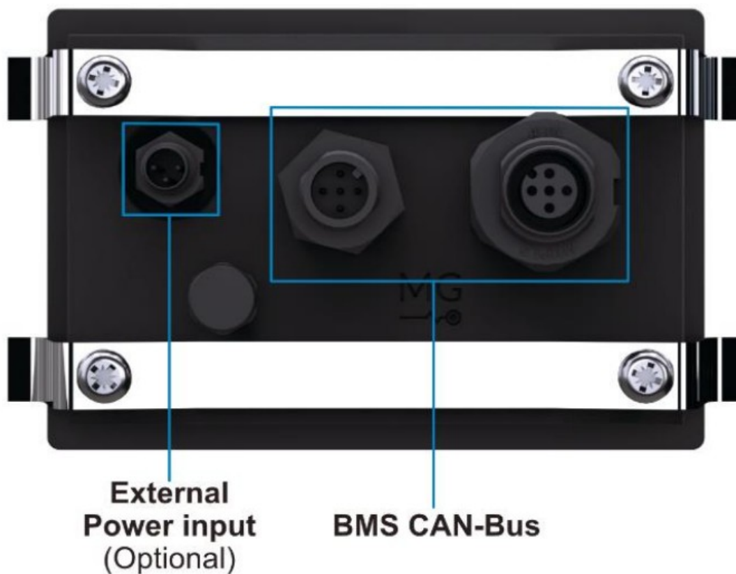
Figure 4 - Energy Monitor rear view
