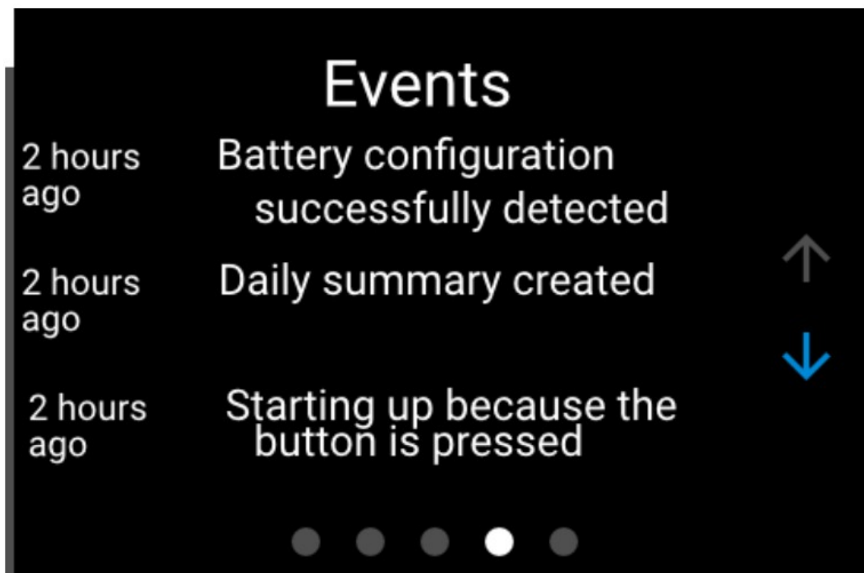
Figure 10 - Events page
