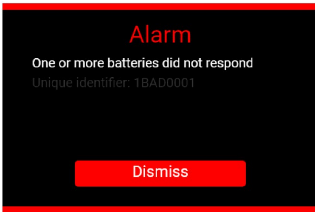
Figure 12 - Pop-up page
