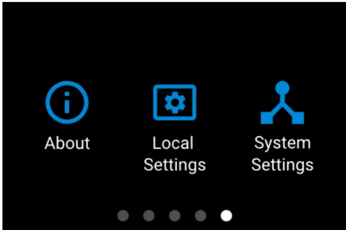
Figure 11 - Settings page
