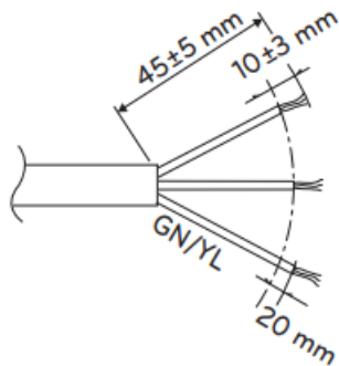
<Sheath removal guide>
