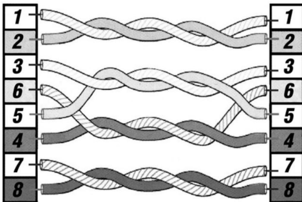
Fig. 5: Description of “Split pairs” error
