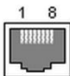
Figure 3. RJ45 Pin Definition
