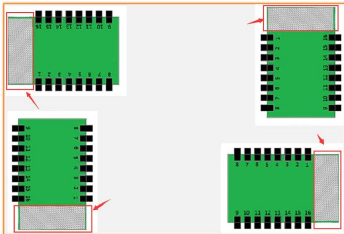
Figure 5. Suggested Module Placement Region
