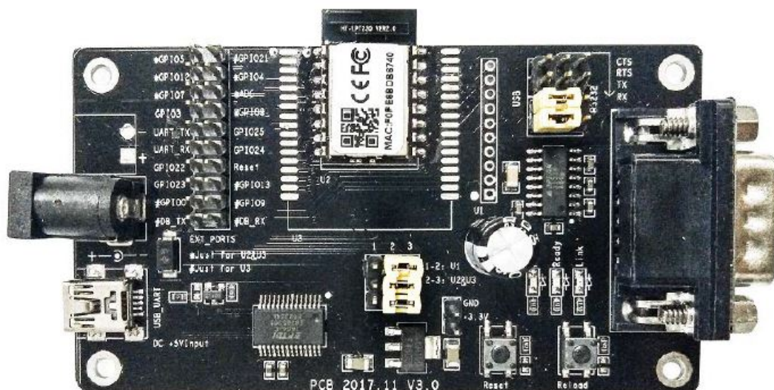
Figure 6. HF-LP271 EVKTypeOne
