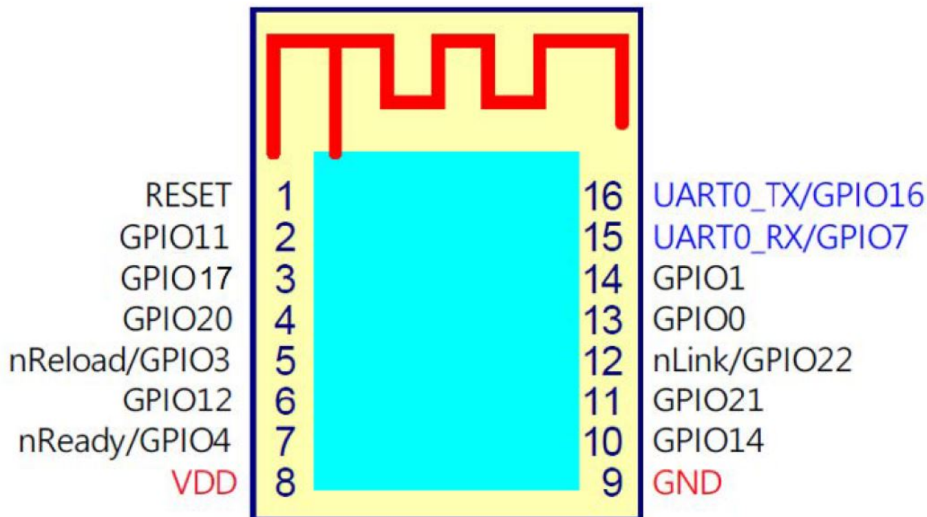
Figure 3. HF-LPT271 Pins Map
