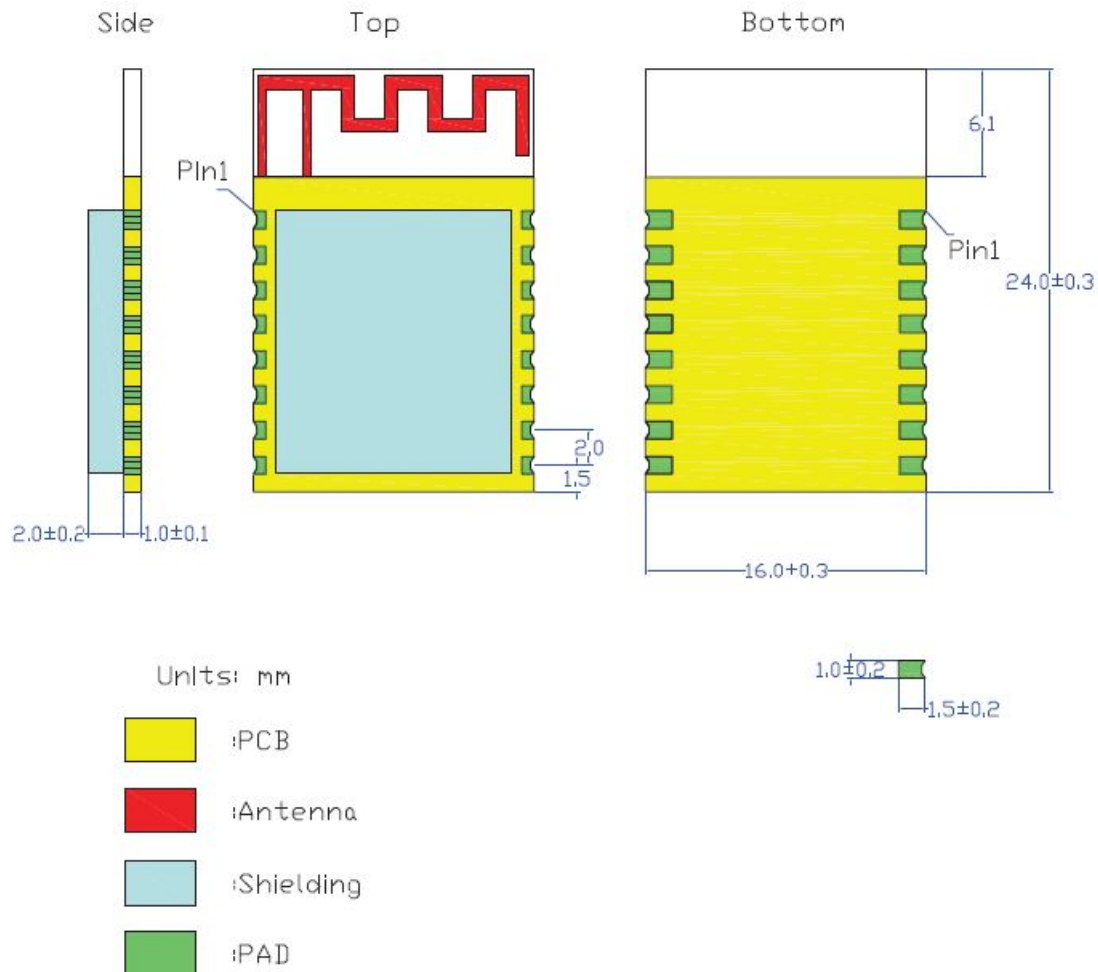
Figure 4. HF-LPT271 Mechanical Dimension
