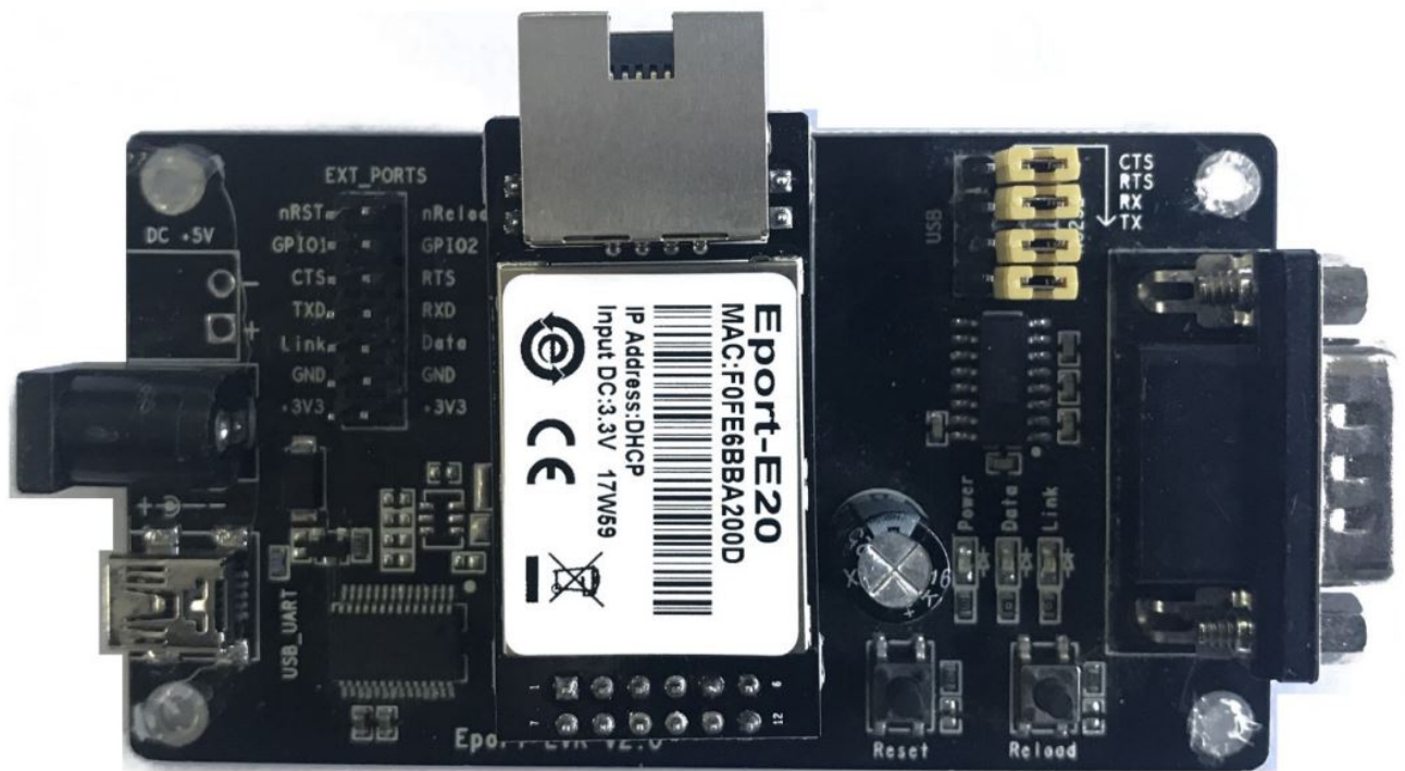
Figure 9. Eport-E20 EVK
