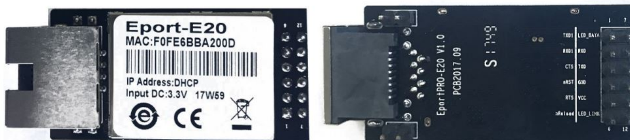
Figure 1. Eport-E20 Appearance
