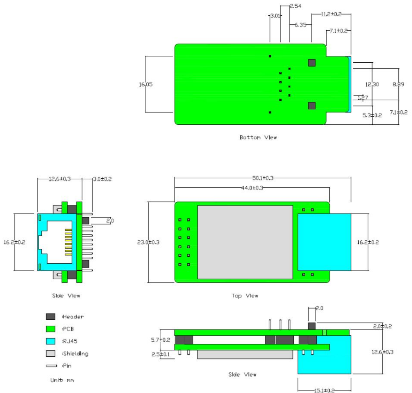
Figure 6. Eport-E20 Mechanical Dimension
