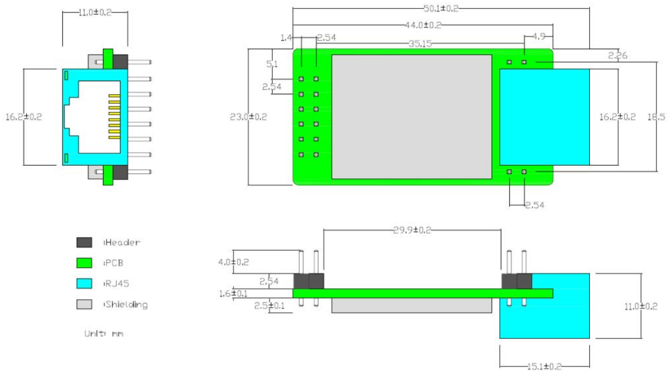
Figure 5. Eport-E20 Mechanical Dimension
