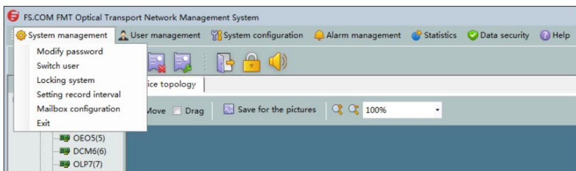
Fig.4.6 System Management
