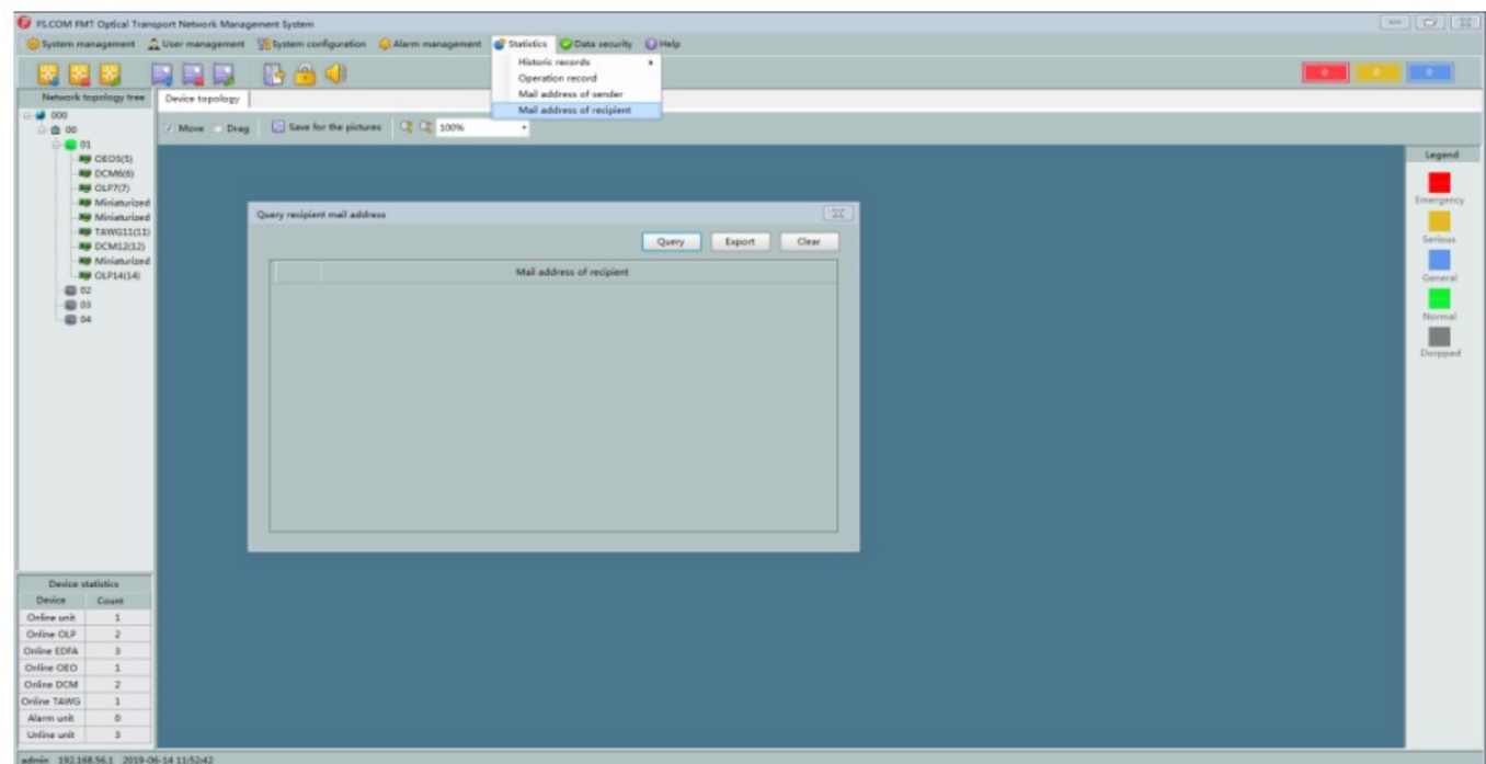
Fig.7.5 Email configuration
