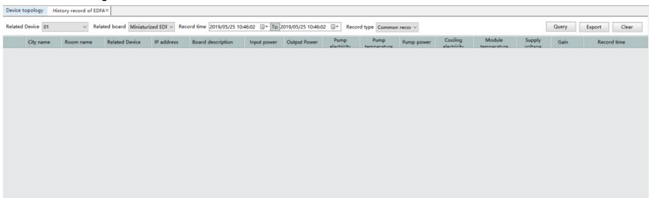
Fig.7.1 History Record
