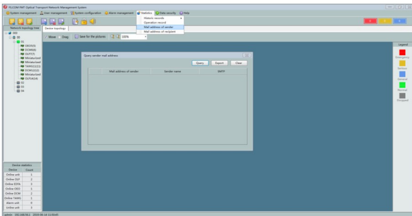
Fig.7.4 Email configuration
