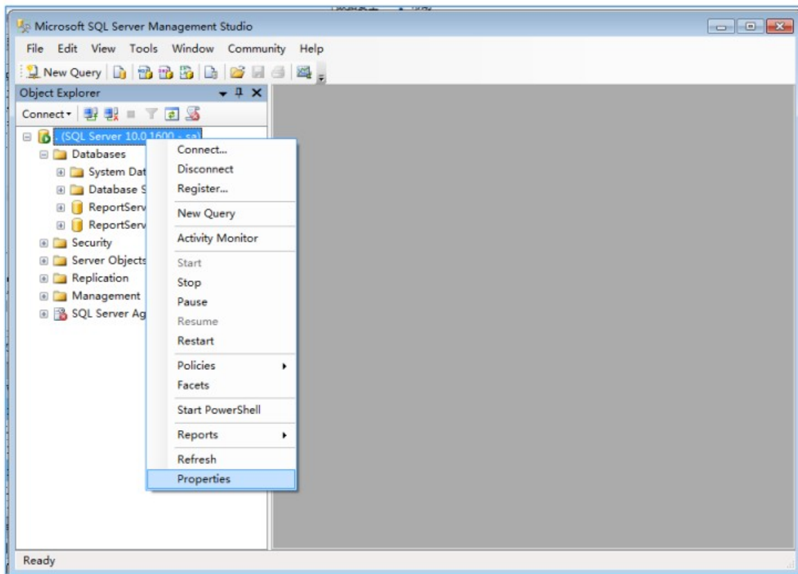
Fig.1.1 Microsoft SSMS
