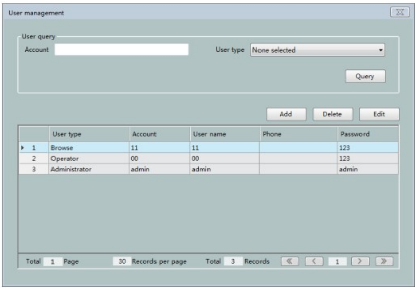
Fig.4.2 User Management
