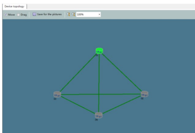
Fig.5.3 Equipment topology
