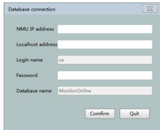
Fig.2.4 Database Connection
