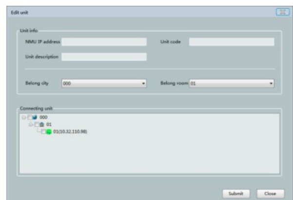
Fig.3.6 Edit unit
