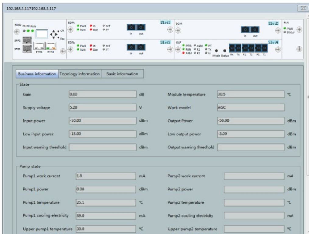
Fig.5.5 EDFA card information
