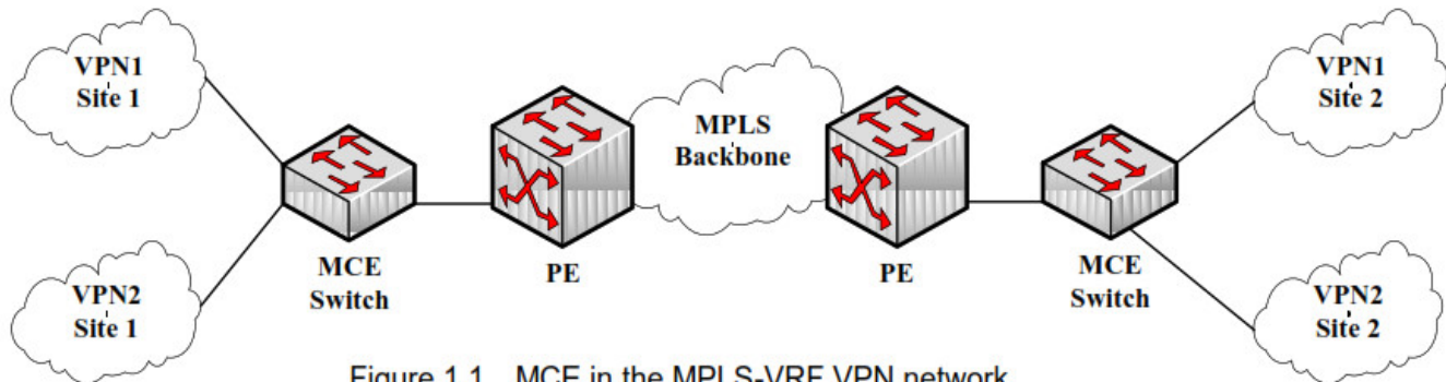
Figure 1.1 MCE in the MPLS-VRF VPN network
