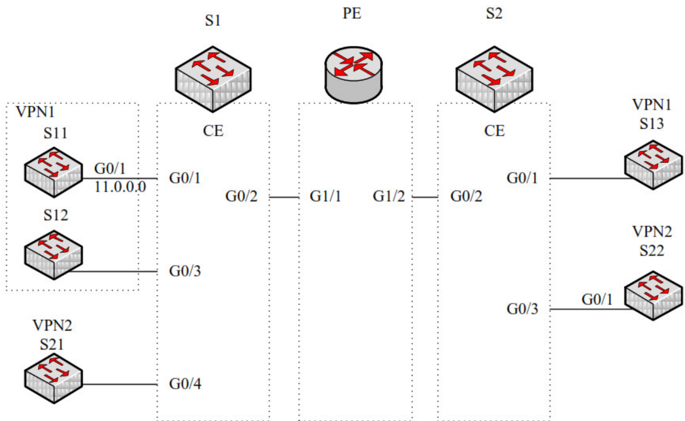
Figure 2.1 MCE configuration example
