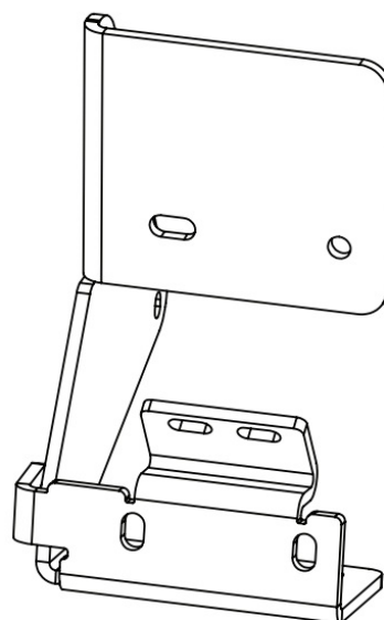
Linkage Mounting Bracket Driver ( Front )
