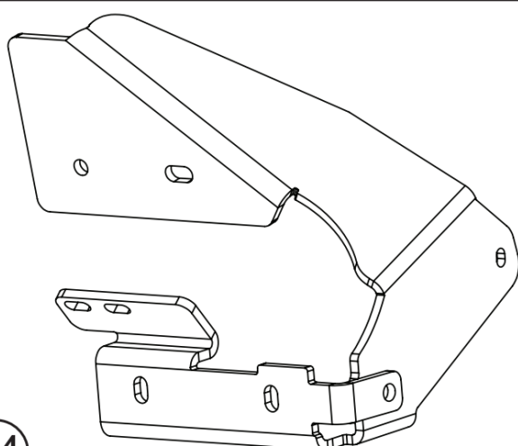
Rail Mounting Bracket Passenger ( Rear )
