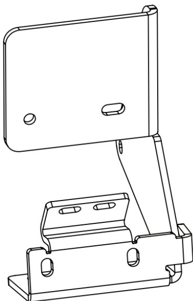
Linkage Mounting Bracket Passenger ( Front )
