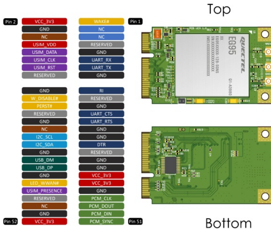
Figure 4. miniPCle Pin Assignment
