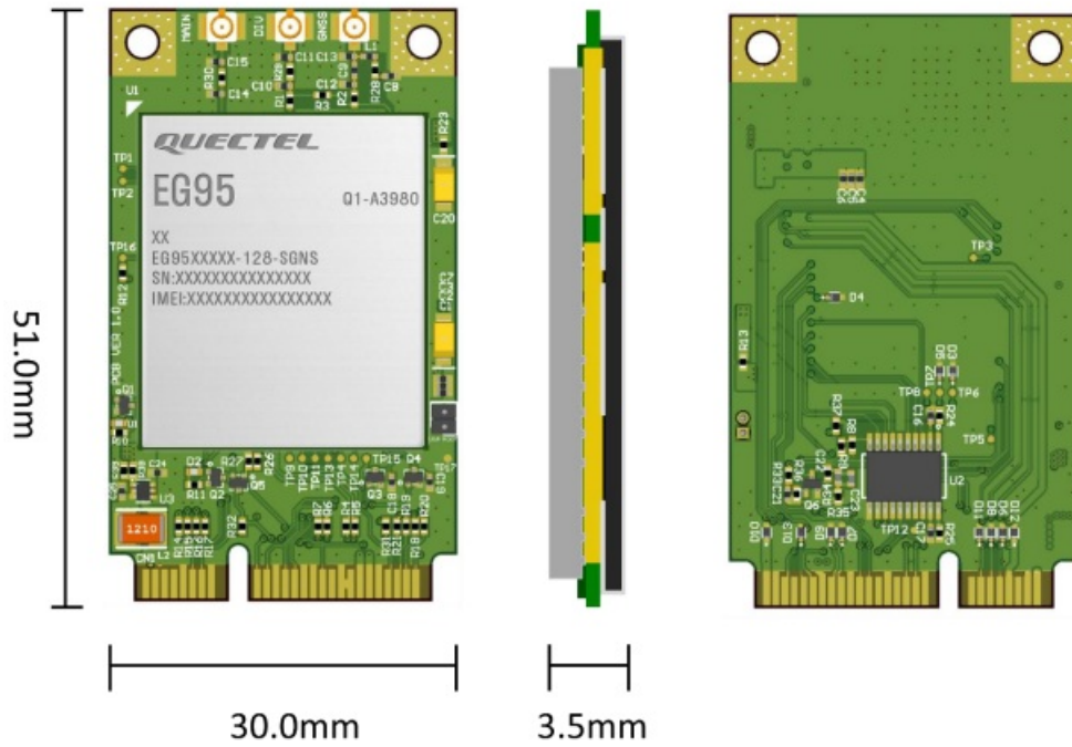
Figure 2. miniPCle EG95 LTE Cat 4 module physical dimension.
