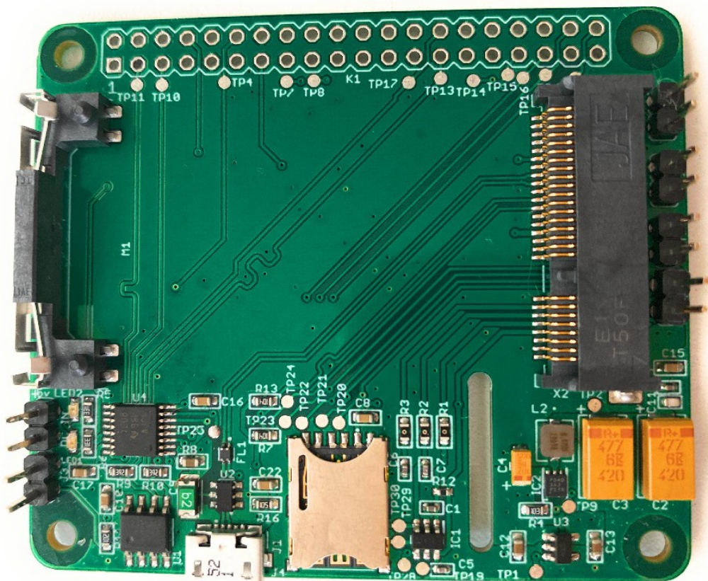
Figure 1. HAT Top View.
