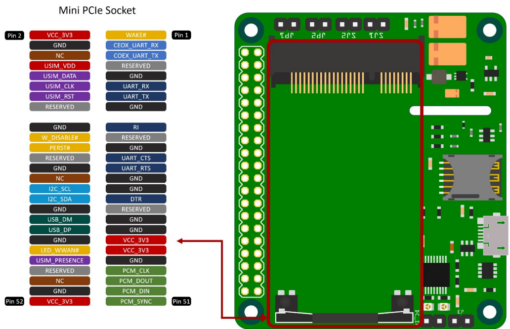
Figure 3. miniPCle Pin Assignment
