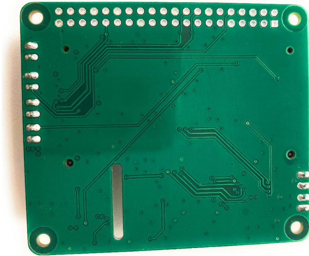
Figure 2. HAT Bottom View.
