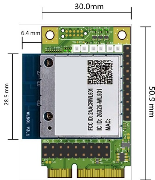
Figure 2: QCA4020 miniPCle Physical Dimension.
