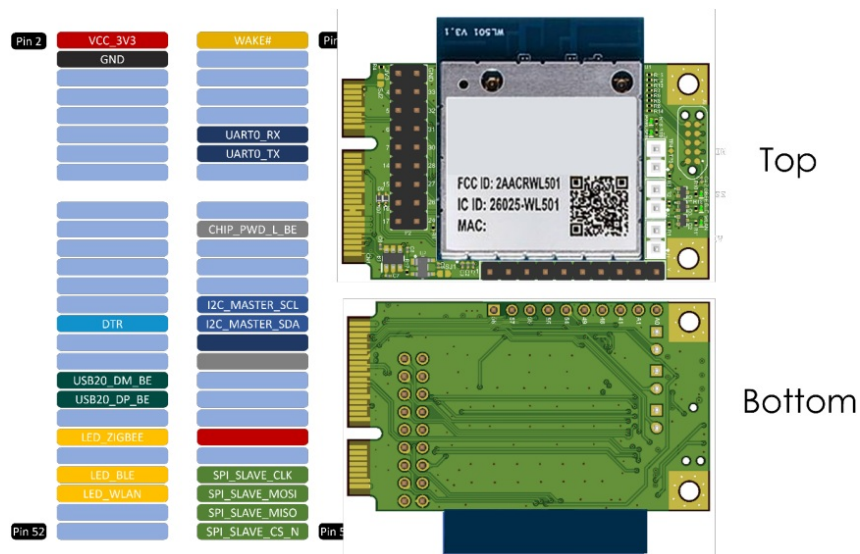
Figure 3: QCA4020 miniPCle Pin out.
