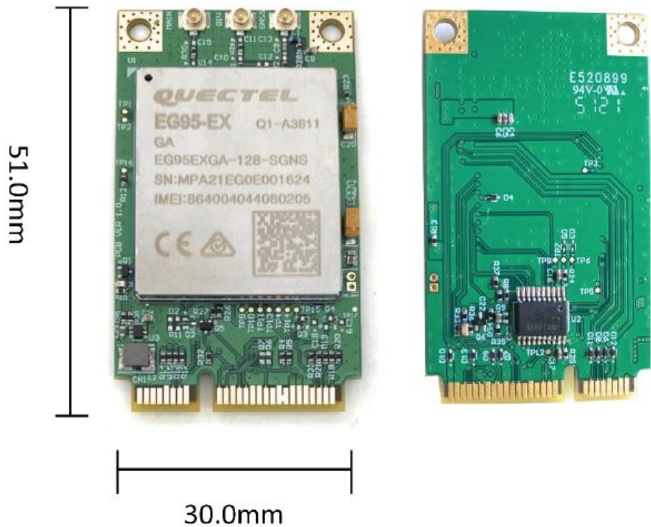
Figure 1. miniPCle EG95 LTE Cat 4 module.
