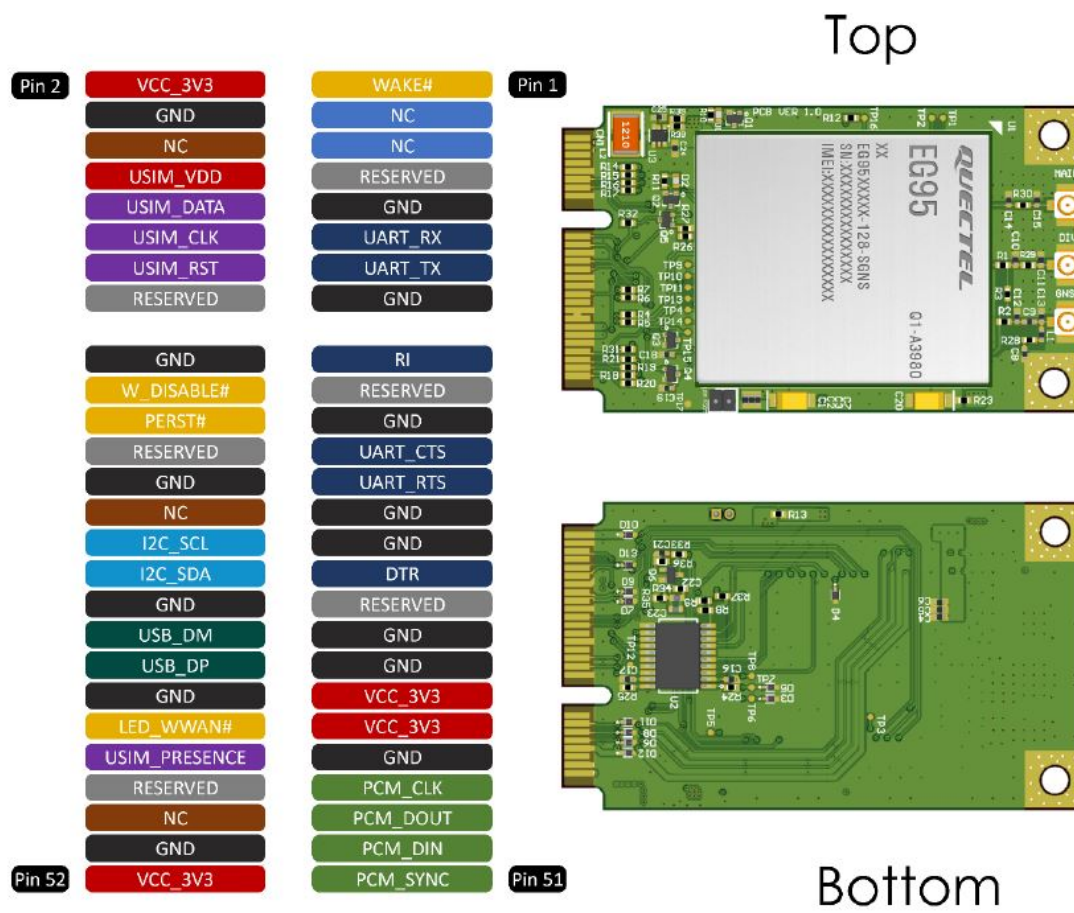
Figure 4. miniPCle Pin Assignment
