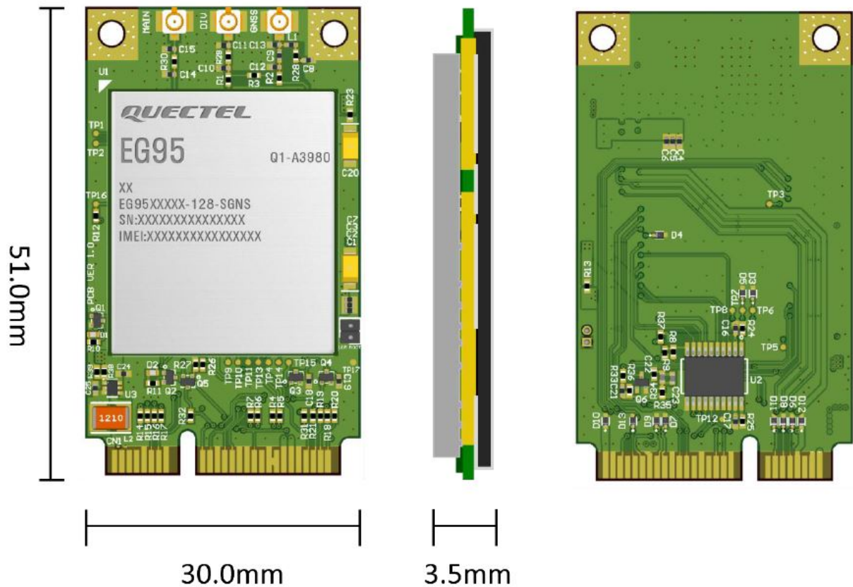
Figure 1. miniPCle EG95 LTE Cat 4 module.
