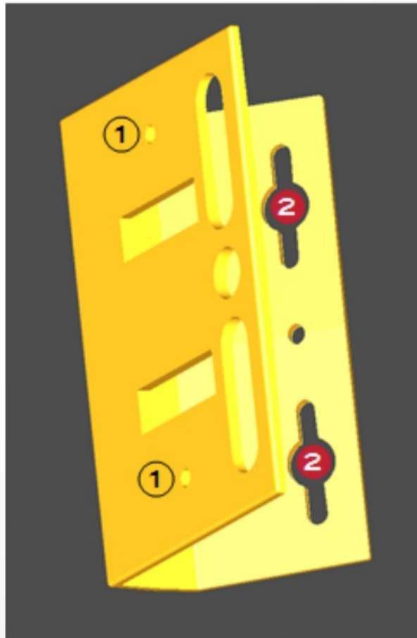
Figure 1-2: Corner Mount Bracket
